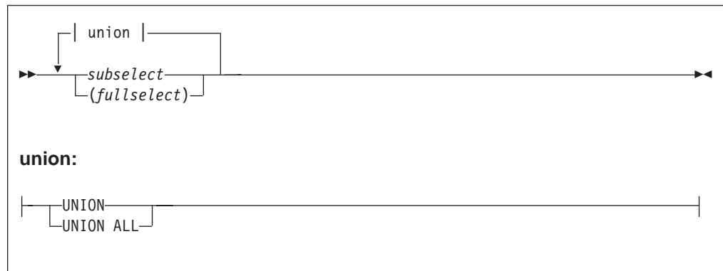
Figure 6. Format of the Fullselect
