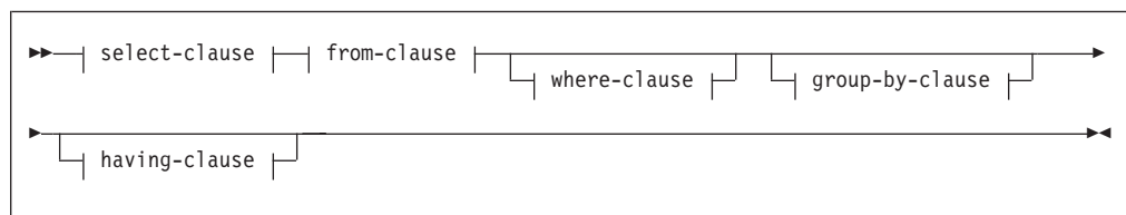
Figure 5. Format of the Subselect
