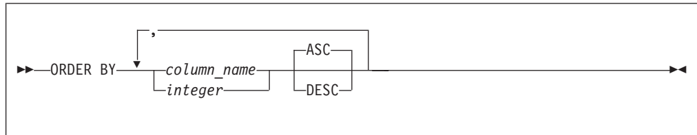
Figure 13. Format of the ORDER BY Clause
