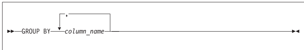
Figure 11. Format of the GROUP BY Clause
