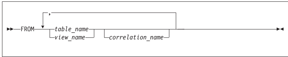
Figure 9. Format of the FROM Clause
