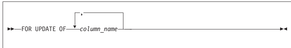
Figure 14. Format of the UPDATE clause
