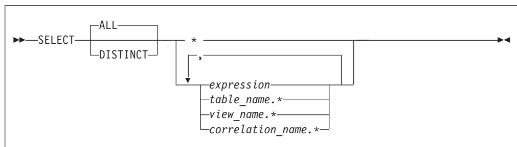
Figure 8. Format of the SELECT clause
