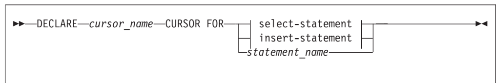
Figure 16. Format of the DECLARE CURSOR statement
