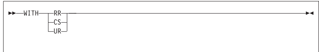
Figure 15. Format of the WITH clause
