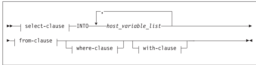
Figure 18. Format of the SELECT INTO statement
