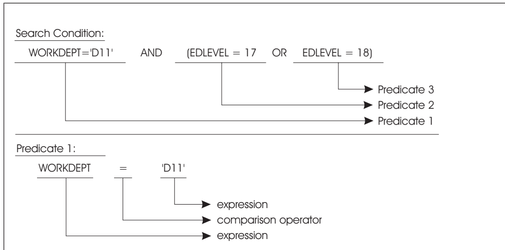
Figure 19. Breakdown of Search Conditions and Predicates
