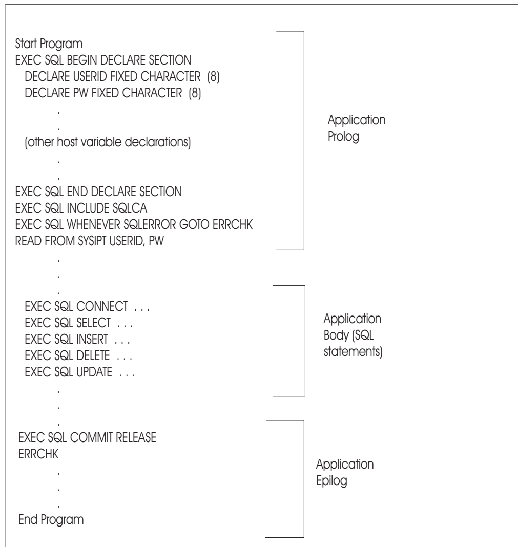
Figure 3. Pseudocode Framework for Coding Programs
