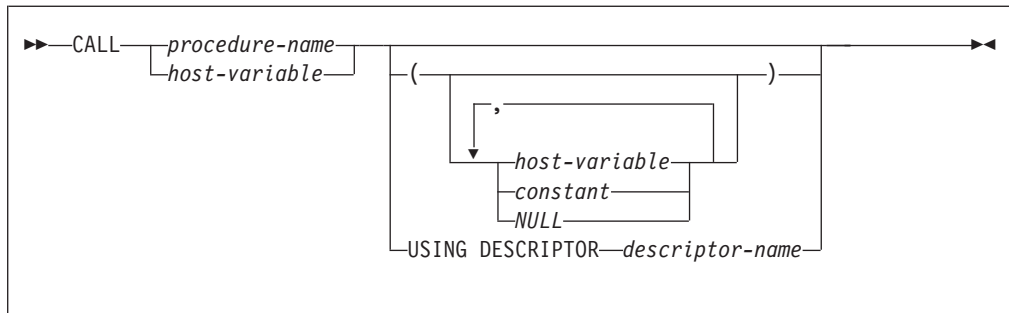
Figure 23. Syntax of SQL CALL statement
