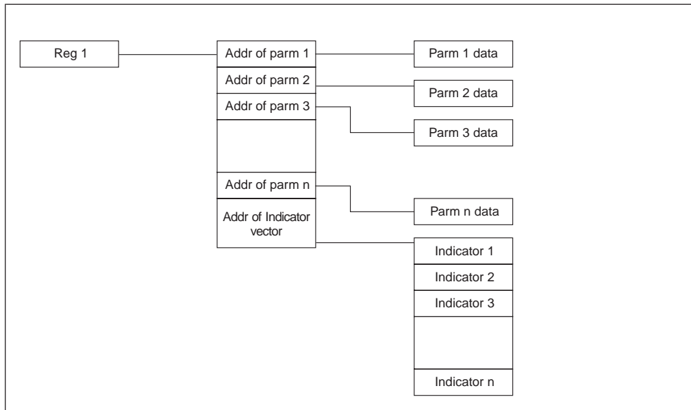
Figure 25. GENERAL WITH NULLS parameter list
