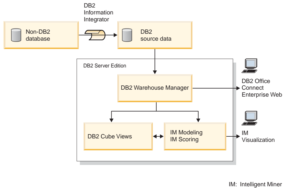
Figure 1. Collecting and analyzing data with the product components of the DB2 Data Warehouse Enterprise Edition
