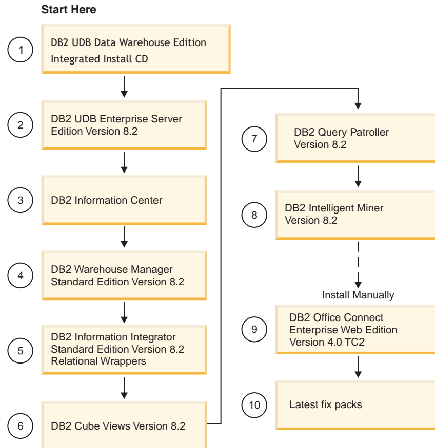
Figure 2. Order of installation for the DB2 Data Warehouse Enterprise Edition
