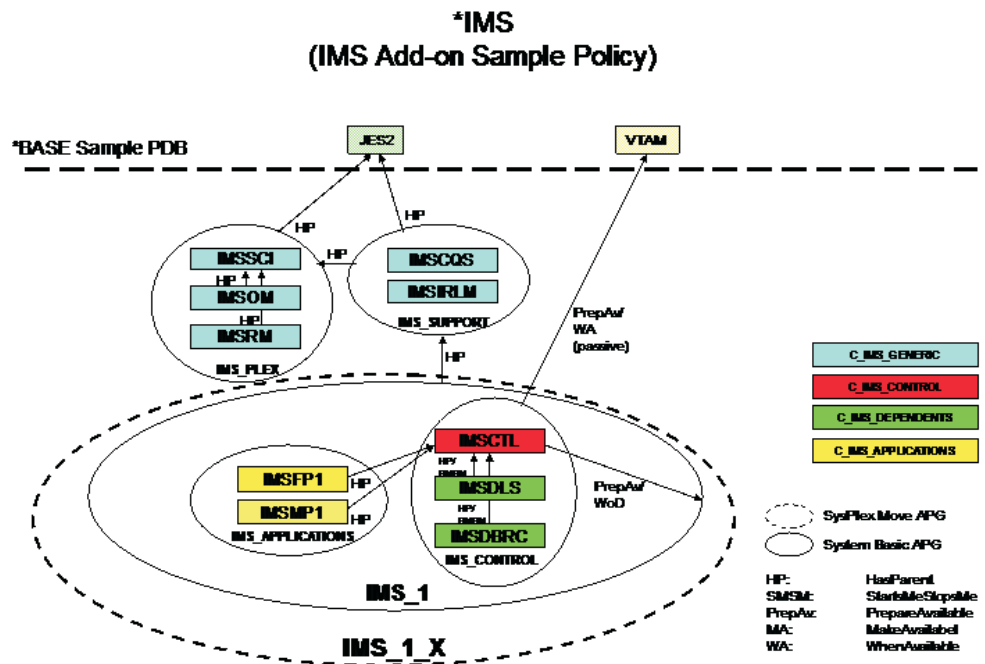
Figure 1. *IMS Add-On Policy
