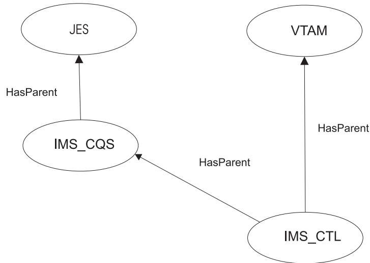
Figure 4. Relationships for IMS CQS
