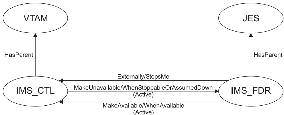
Figure 3. Relationships for IMS FDR
