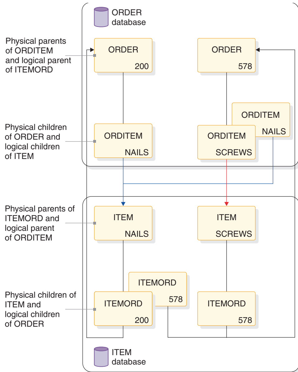
Figure 75. Two unidirectional logical relationships
