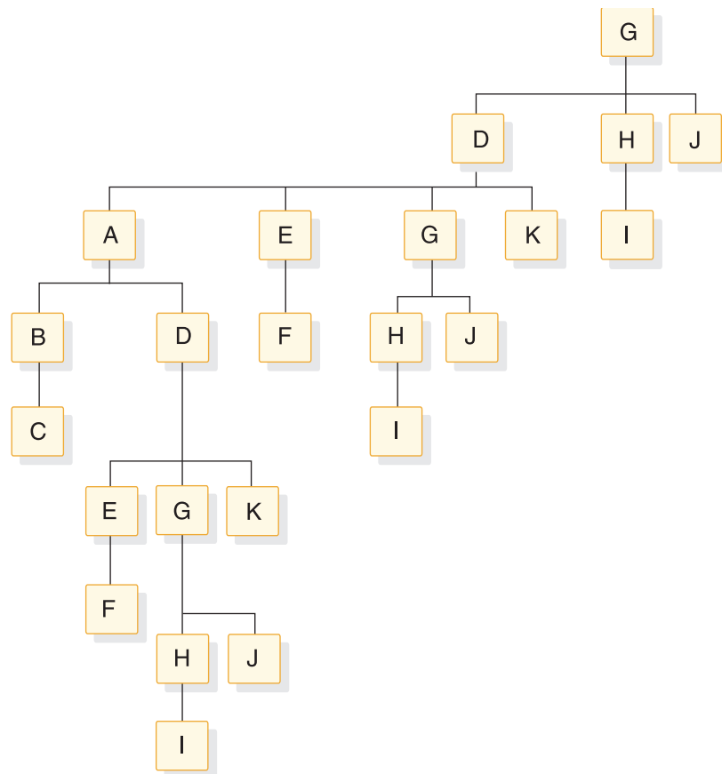
Figure 176. Secondary index structure indexed in secondary index on segment G
