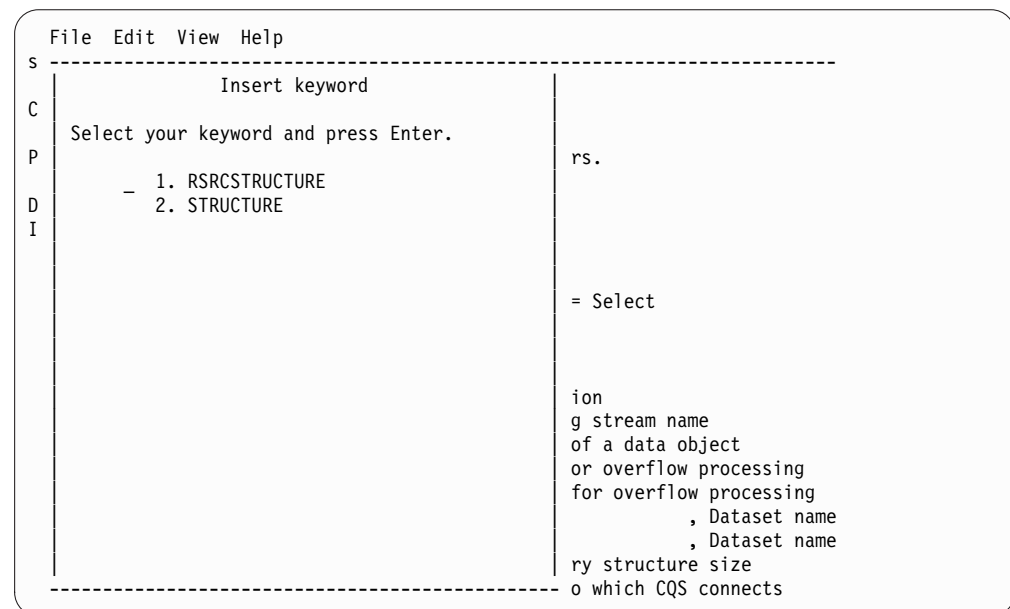
Figure 47. Example of insert pop-up window for Syntax Checker Keyword Display panel
