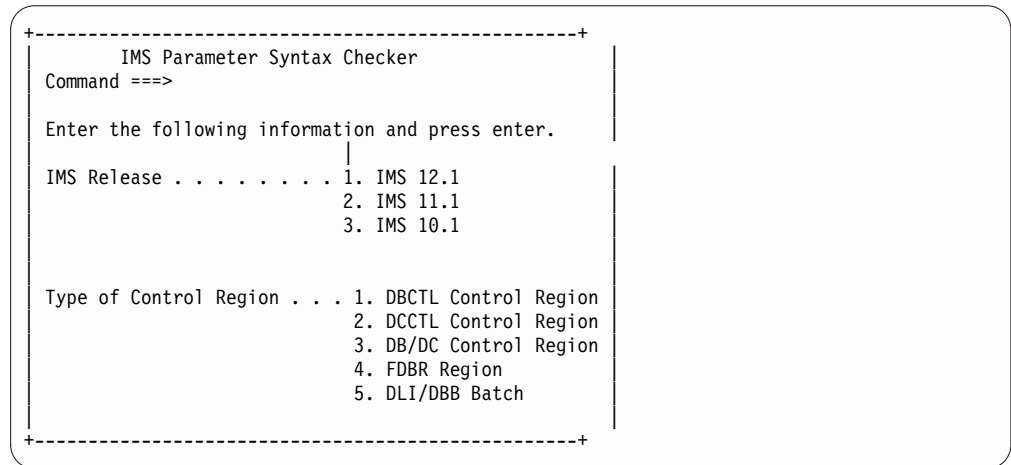
Figure 52. IMS Parameter Syntax Checker panel
