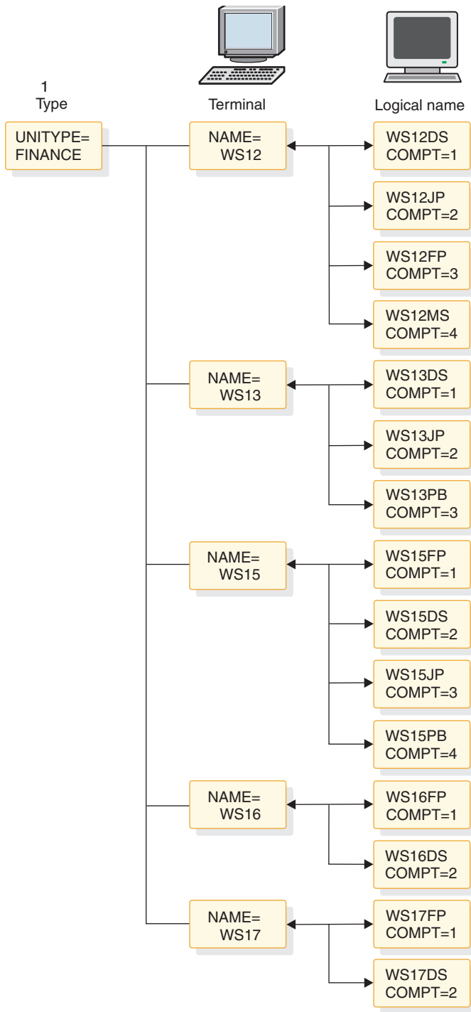
Figure 32. Finance Communication system. 1 Can also specify UNITYPE=3601.
