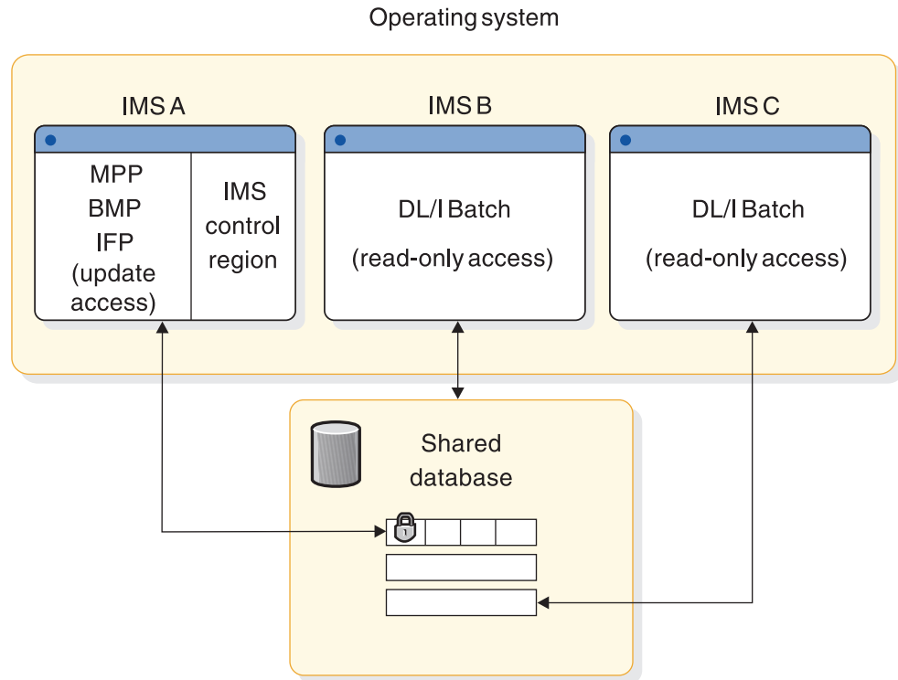
Figure 39. Data sharing at the database level with update access
