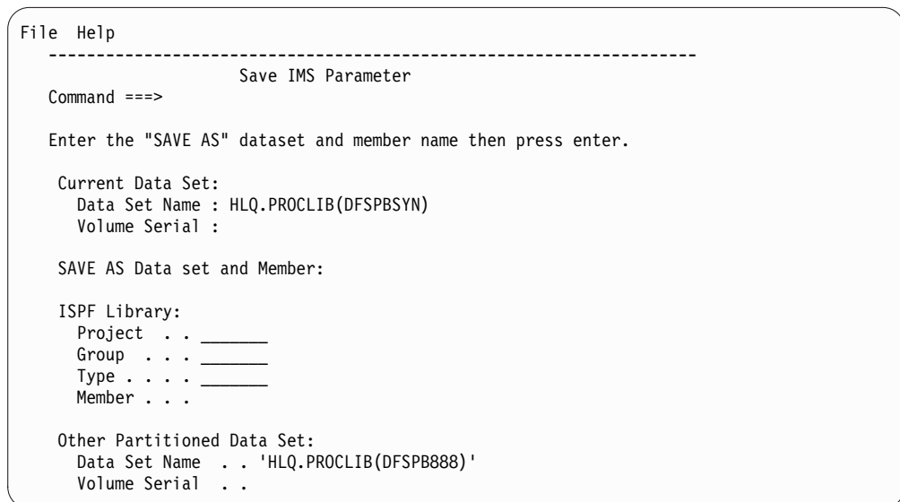
Figure 51. SAVE AS Prompt panel
