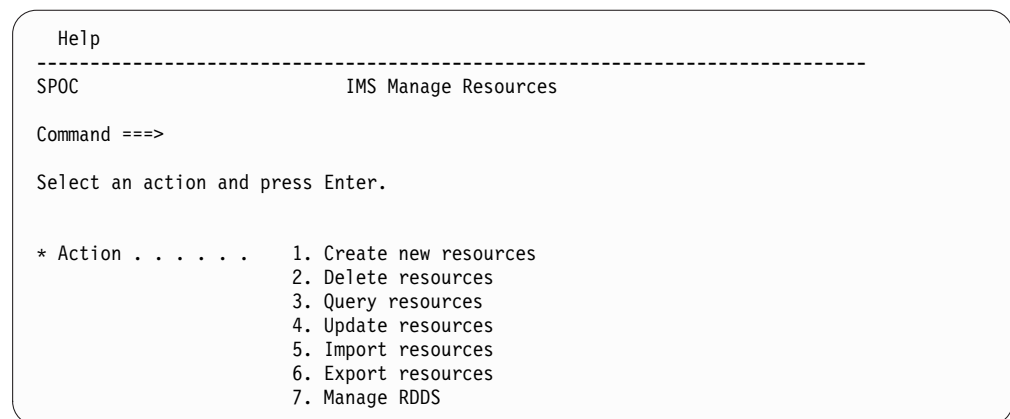
Figure 7. IMS Manage Resources main panel
