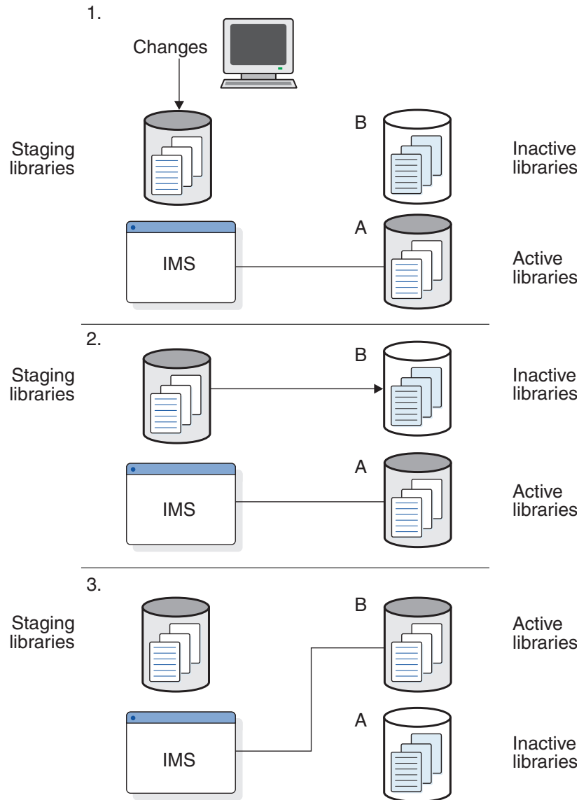
Figure 12. How libraries are used when you change your system online
