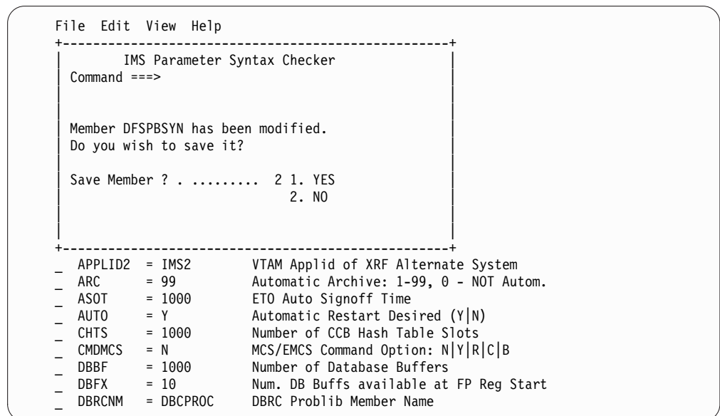
Figure 50. Save Member Prompt panel
