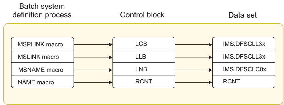
Figure 6. Control block generation process for MSC resources
