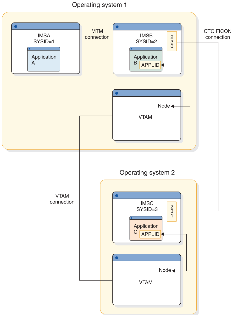
Figure 38. Multiple Systems Coupling example
