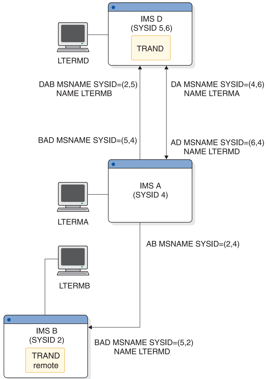
Figure 117. Remote LTERMs
