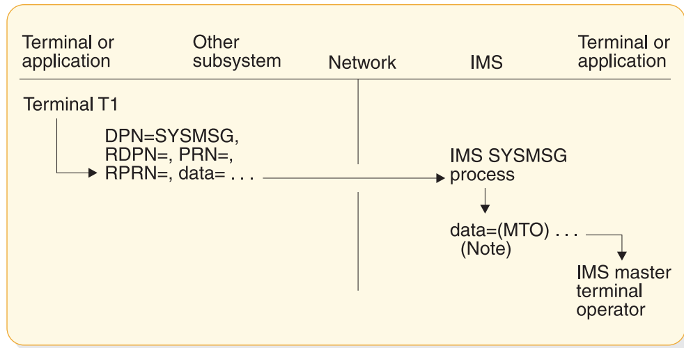
Figure 72. Example of SYSMMSG without PRN from other subsystem terminal to IMS A
