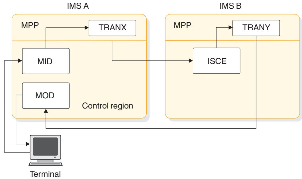
Figure 64. ISC example for IMS-to-IMS application routing with MFS
