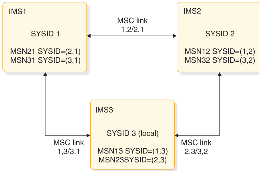
Figure 119. MSC network without an IMSplex
