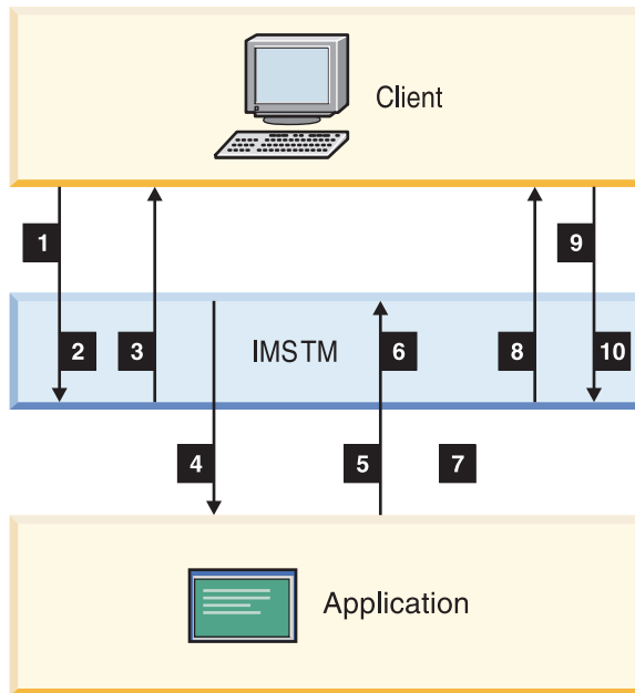
Figure 142. Commit-then-send (IMS standard) flow
