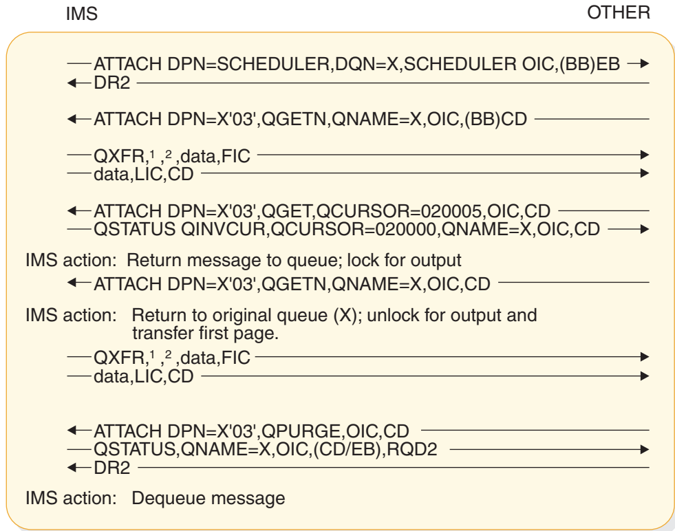
Figure 93. Example of demand-paged SCHEDULER output, OLP defined, QGET by cursor request for a page not within the range of output message
