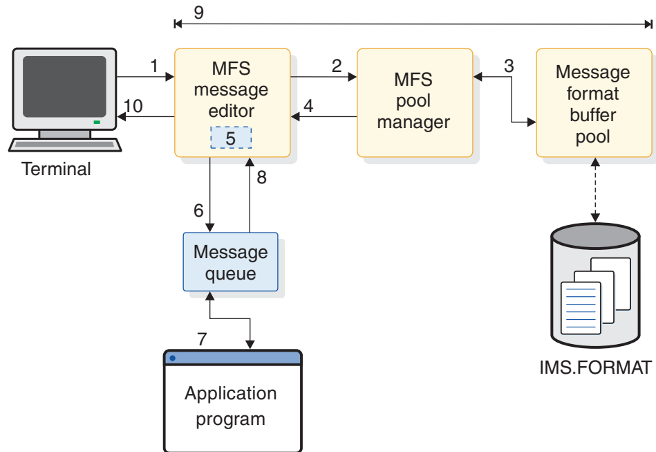
Figure 49. Overview of the MFS online environment
