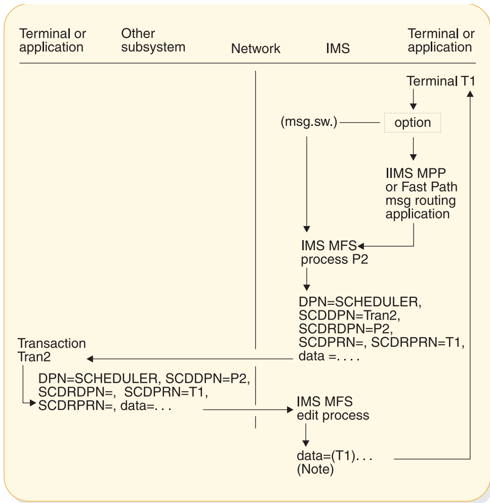
Figure 78. Example of message routing with IMS MFS
