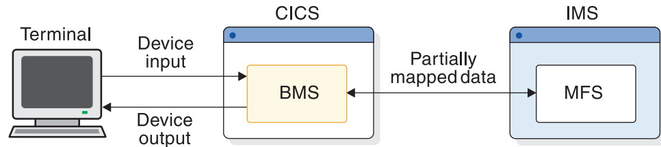
Figure 55. IMS MFS DPM mapping function distributed to CICS's BMS
