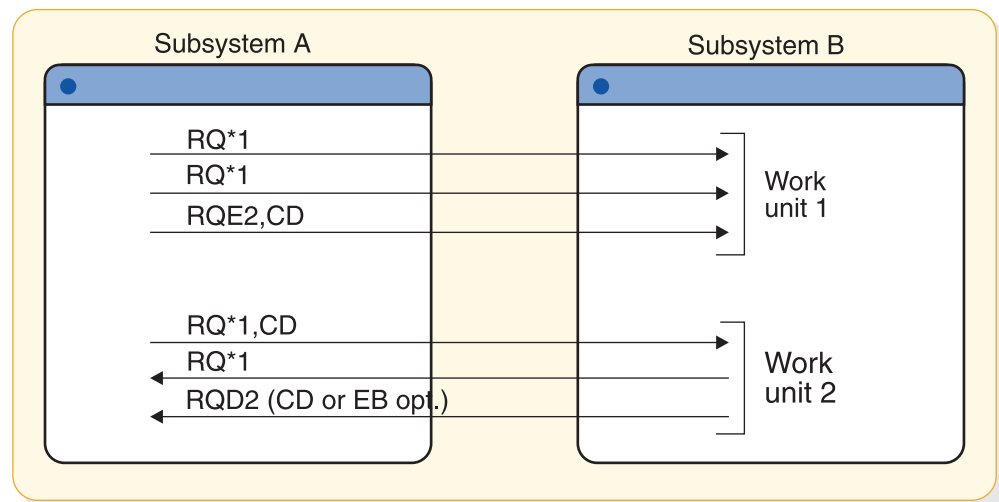
Figure 67. Work unit examples
