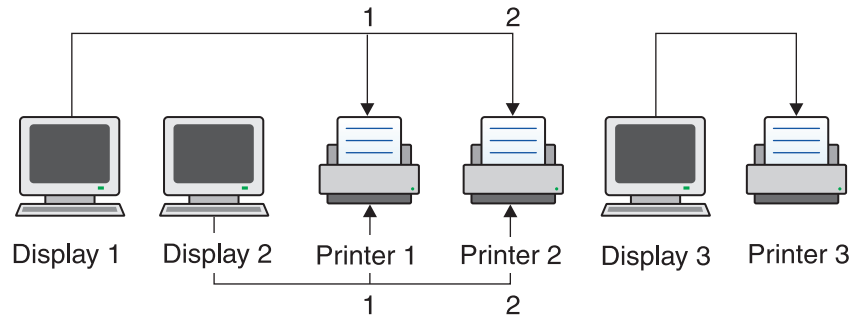
Figure 52. Sequence of IMS TERMINAL macros
