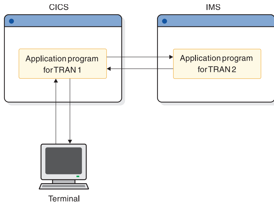
Figure 79. Synchronous processing with SEND and RECEIVE
