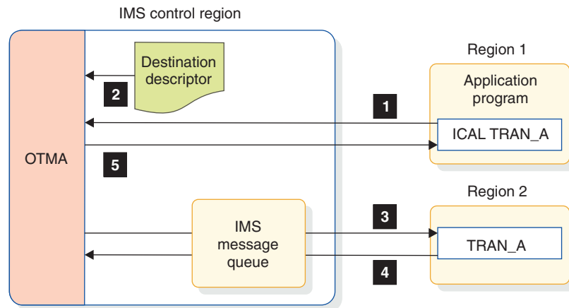
Figure 153. IMS synchronous program switch processing
