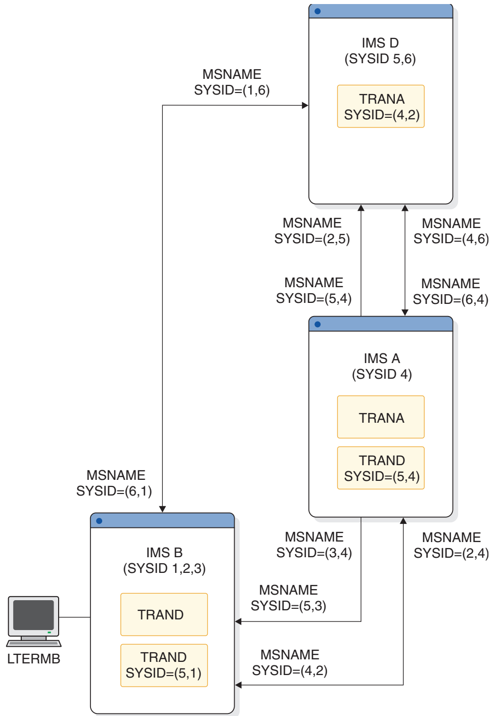
Figure 116. Message routing
