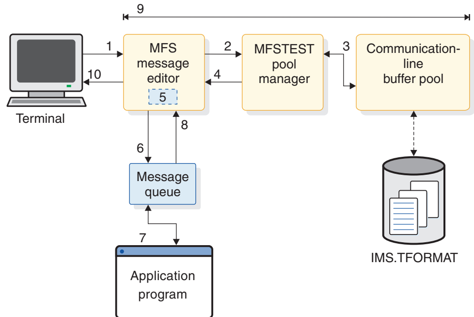
Figure 50. Overview of the MFS test environment
