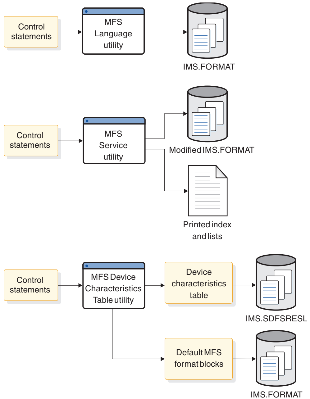
Figure 48. MFS utilities and their output
