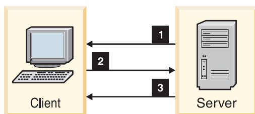
Figure 148. Server-available flow
