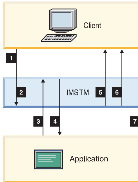
Figure 144. Send-then-commit flow
