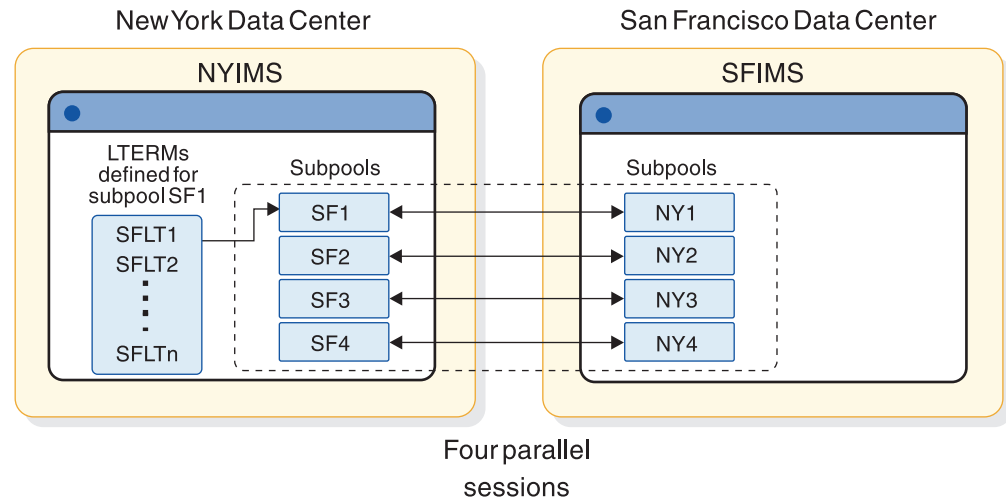
Figure 66. Two IMS systems defined to each other as ISC nodes
