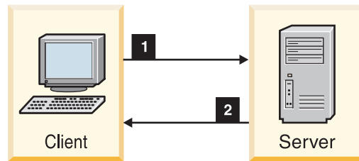
Figure 147. Client-bid flow
