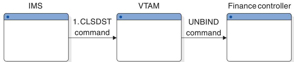
Figure 155. Termination processing
