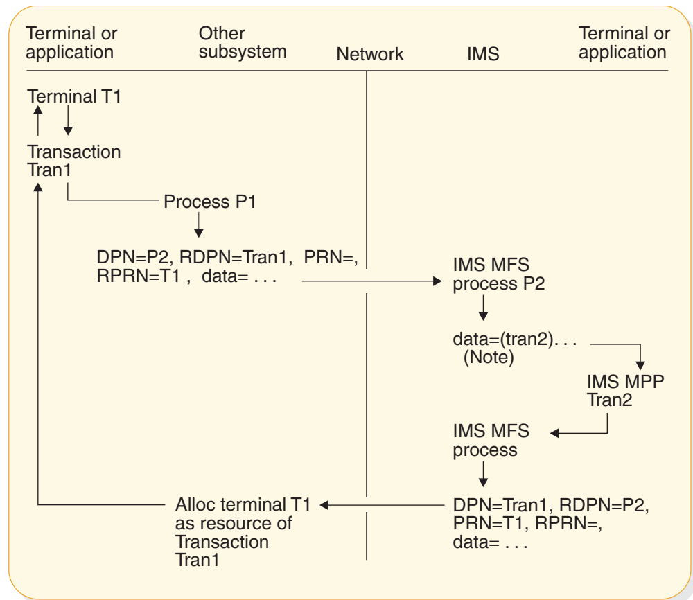
Figure 75. Example of other subsystem terminal accesses IMS application program with reply
