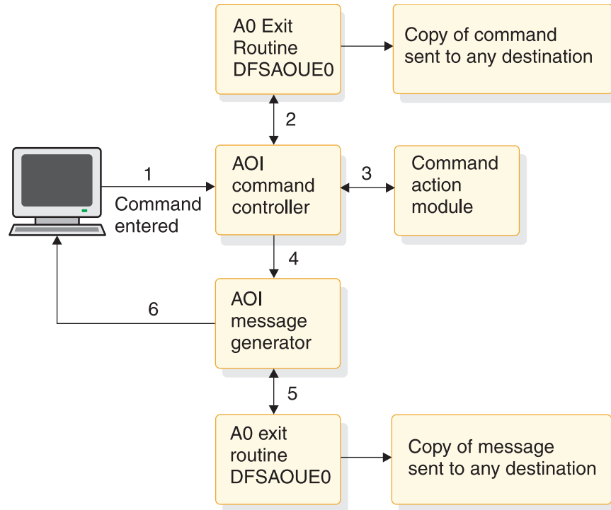
Figure 23. Processing when a command is entered at the terminal
