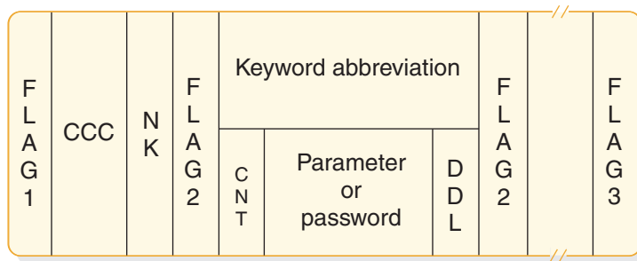
Figure 26. Edited command buffer
