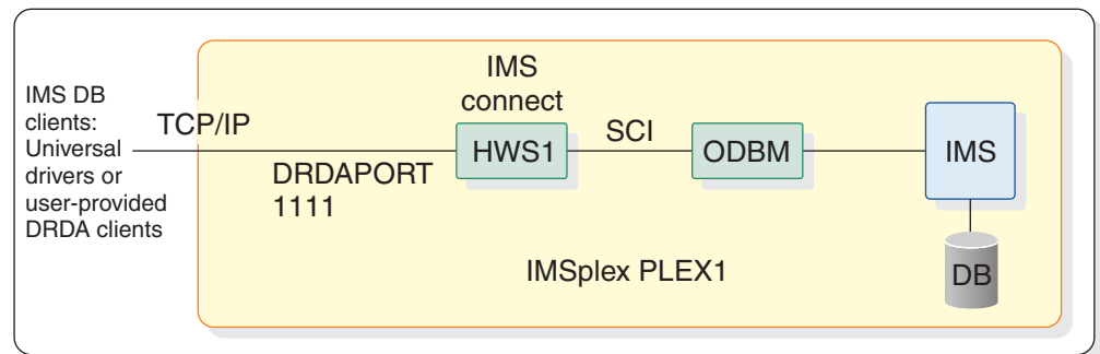
Figure 56. Simple IMS Connect system configuration for IMS DB support
