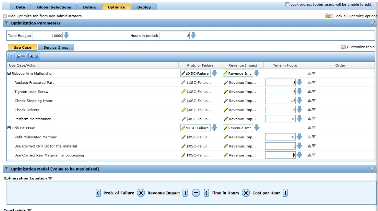
Figure 9. Optimize tab
