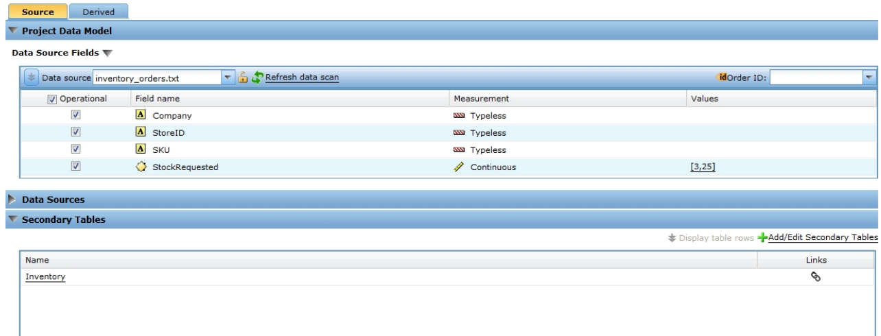
Figure 3. Data tab
