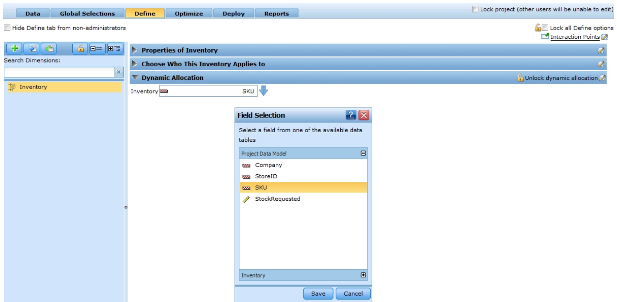
Figure 4. Define tab showing properties for Inventory
