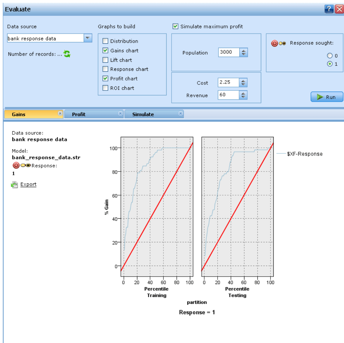
Figure 6-10 Gains chart
