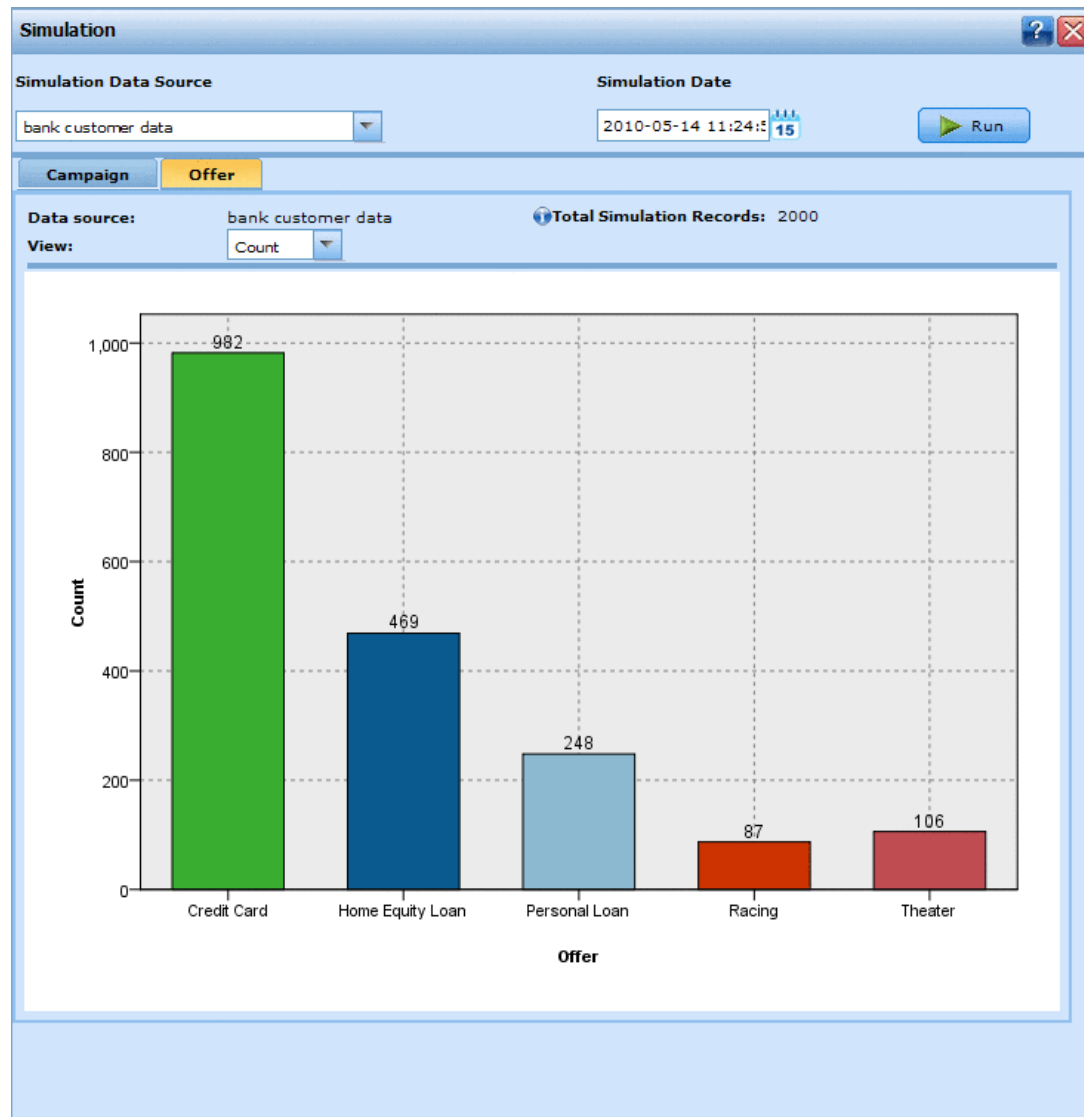
Figure 7-14 Simulation results
