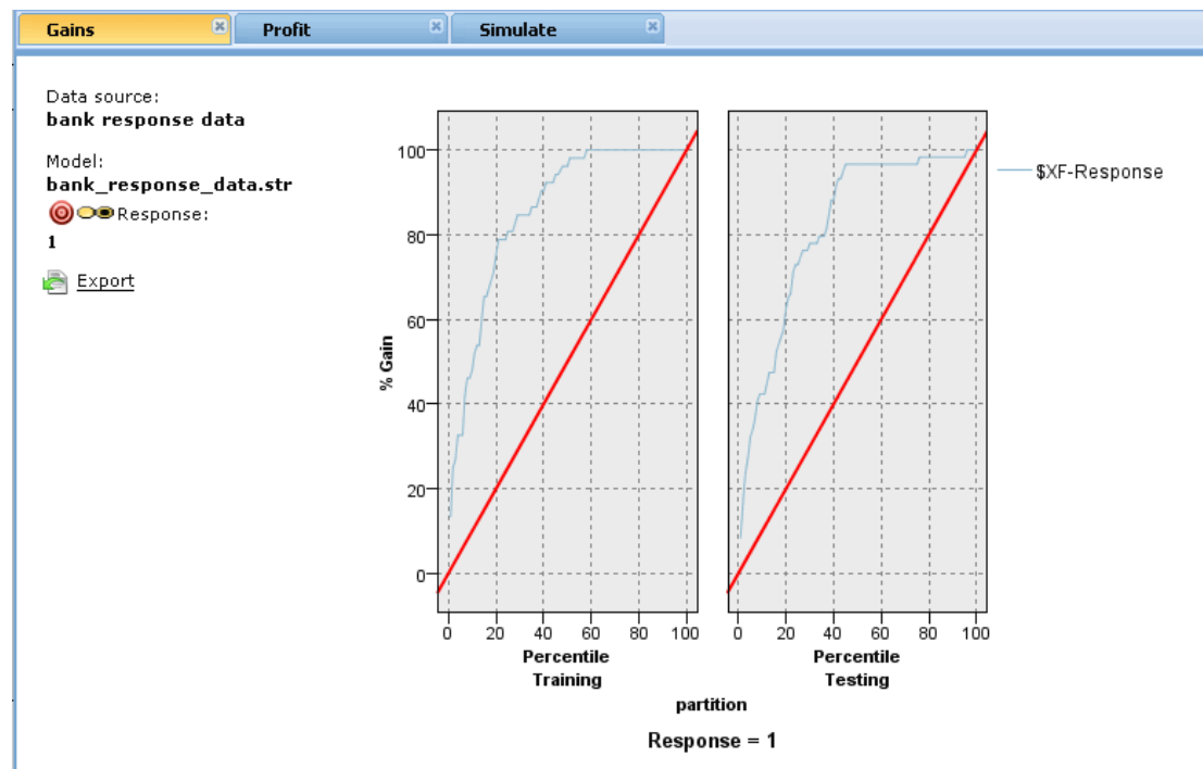
Figure 6-11 Gains chart
