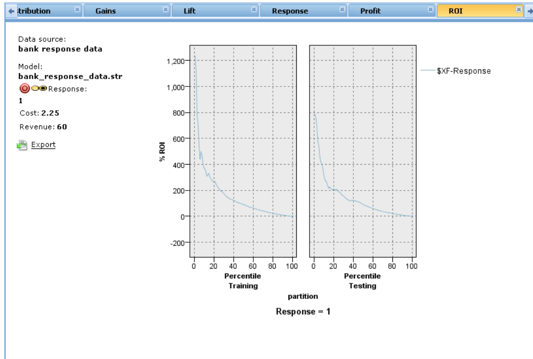
Figure 6-15 ROI chart
