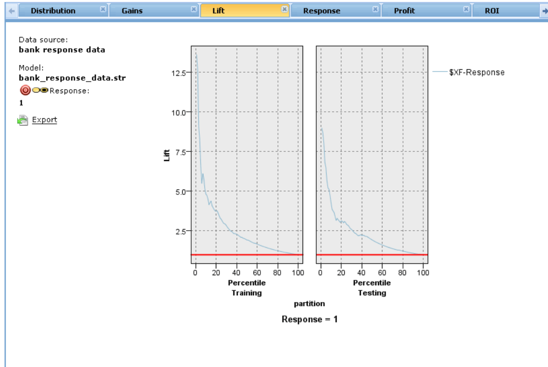
Figure 6-12 Lift chart
