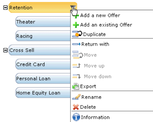
Figure 7-2 Dimension tree
