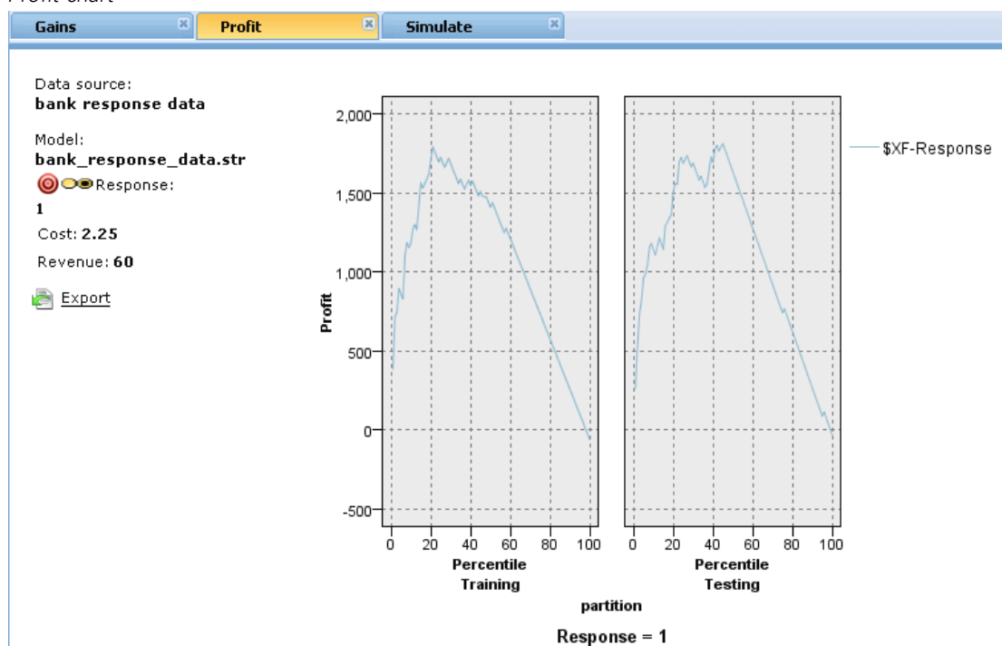
Figure 6-14 Profit chart
