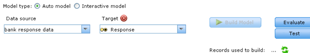
Figure 7-3 Model settings
