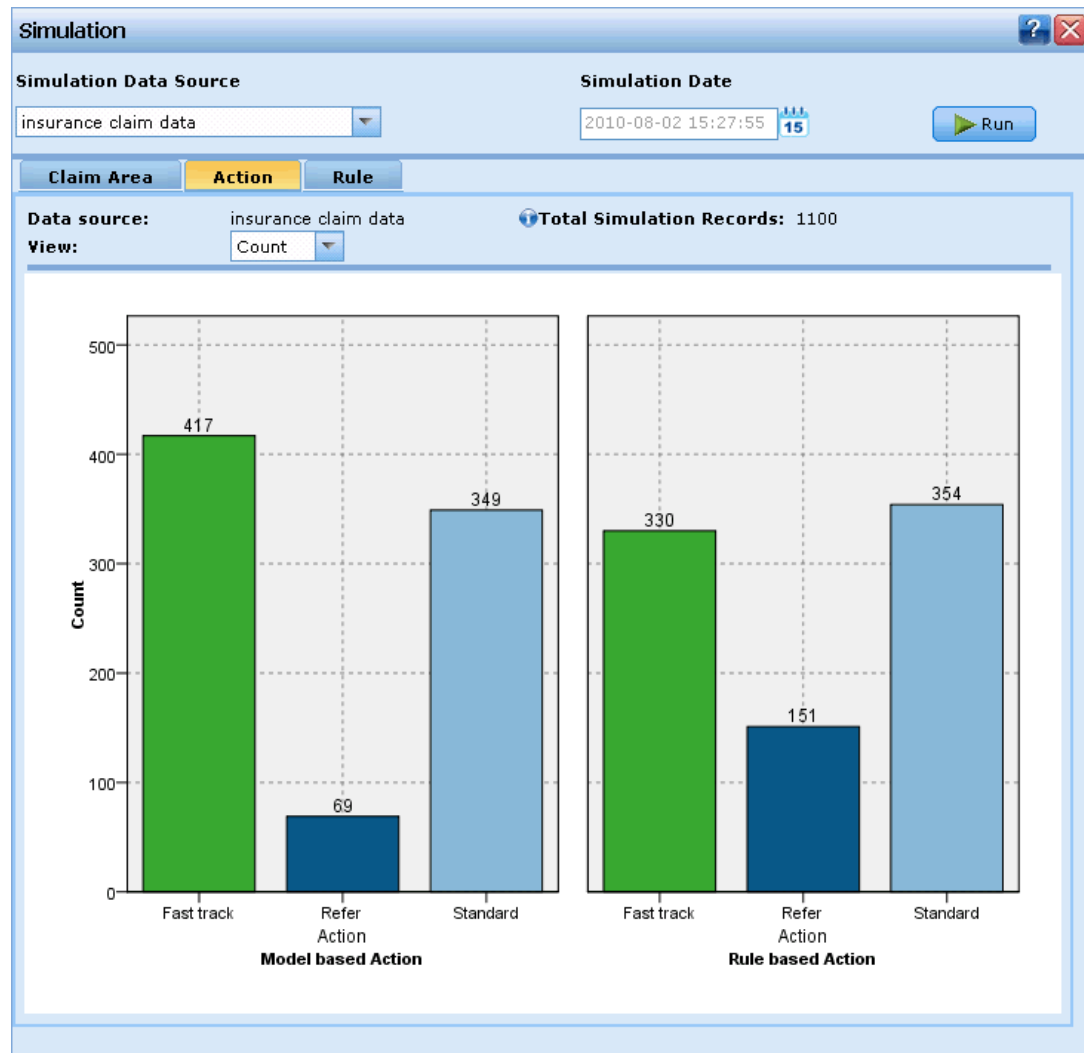
Figure 8-11 Simulation results
