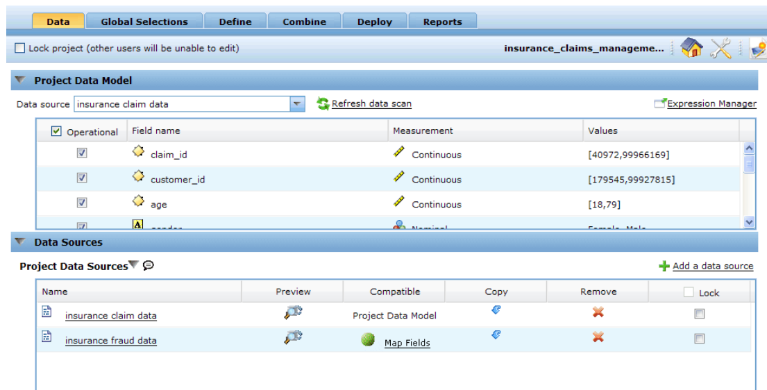
Figure 2-4 Data tab
