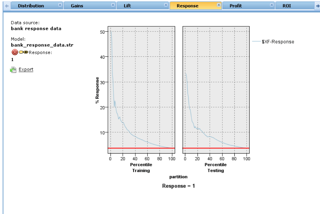
Figure 7-13 Response chart
