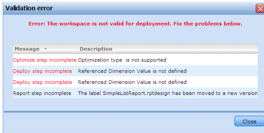
Figure 10-2 Validation errors
