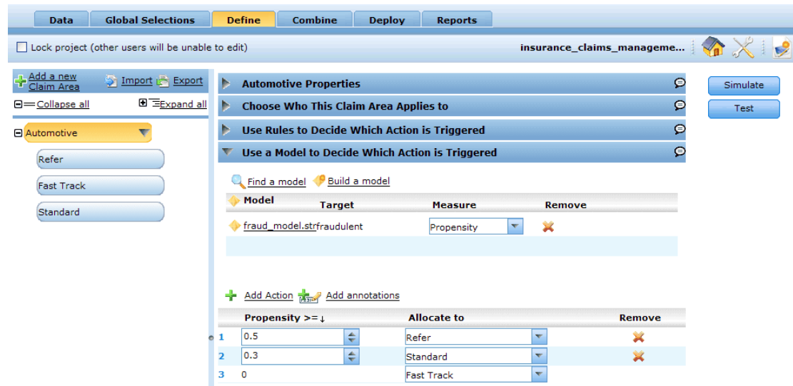
Figure 2-14 Define tab
