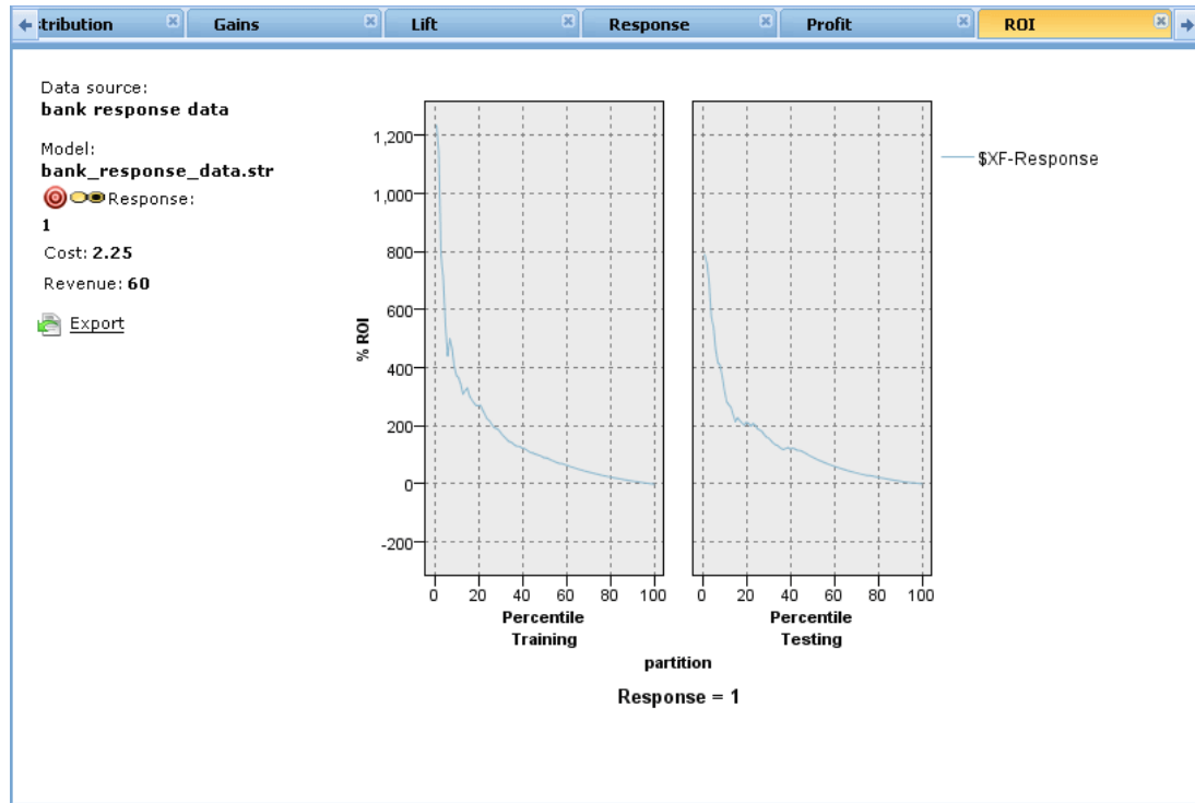
Figure 7-15 ROI chart
