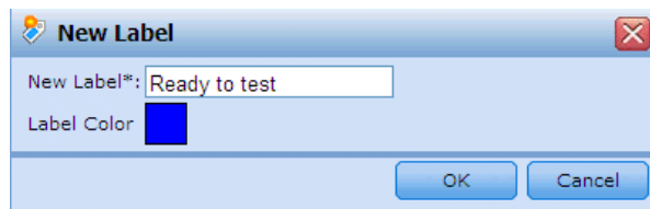
Figure 12-8 New label
