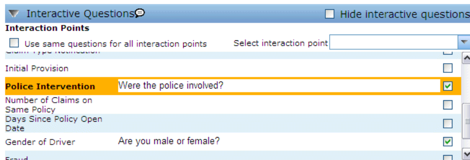
Figure 12-9 Interactive questions
