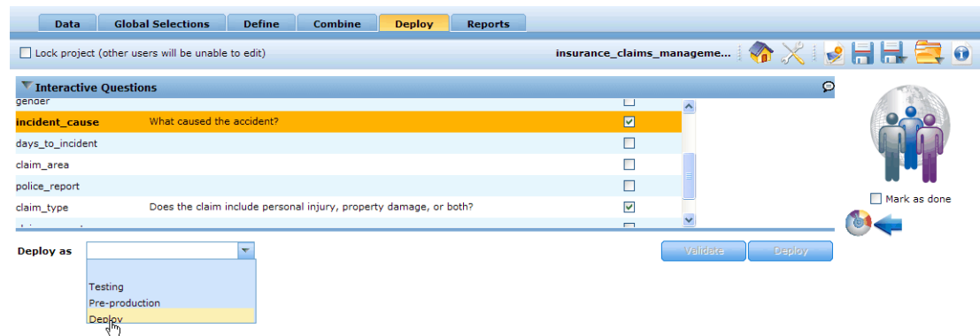
Figure 2-25 Deploy tab
