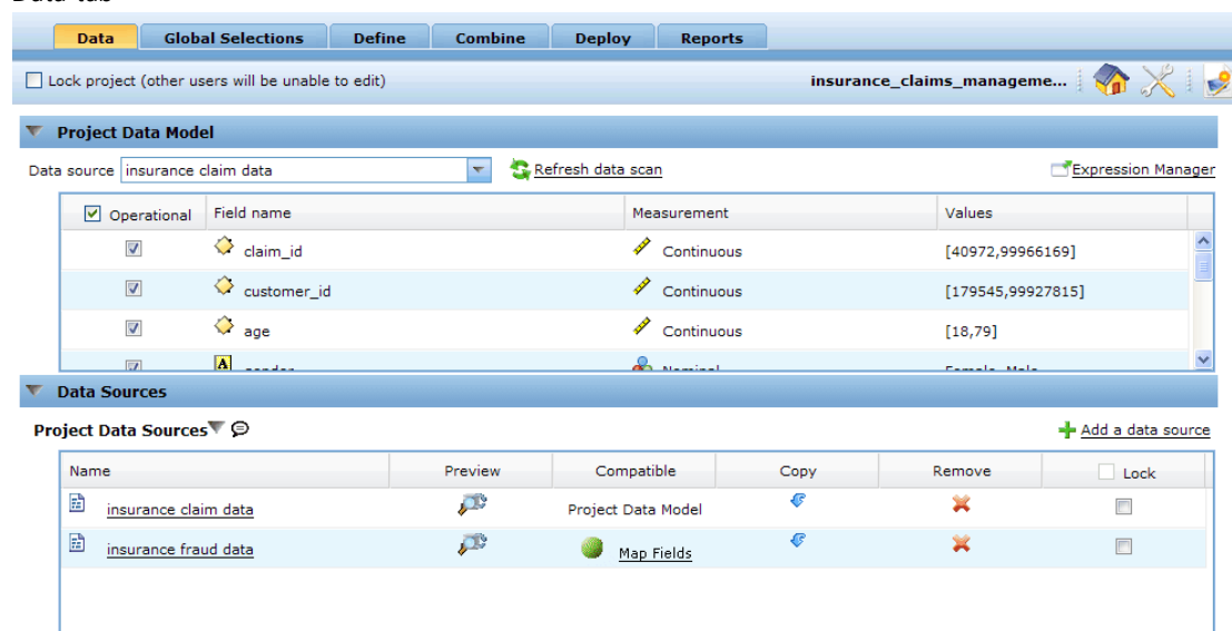
Figure 4-1 Data tab
