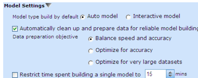
Figure 3-11 Model Settings
