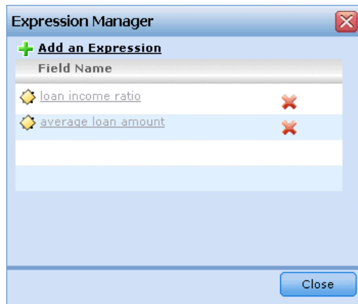
Figure 4-15 Expression manager
