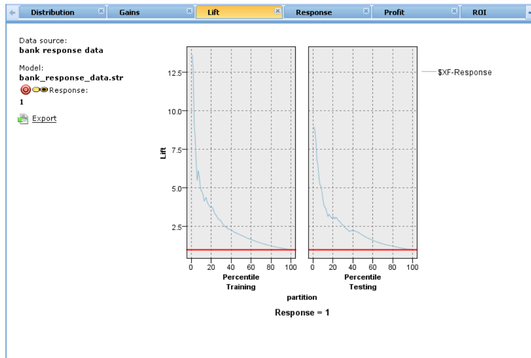
Figure 7-12
