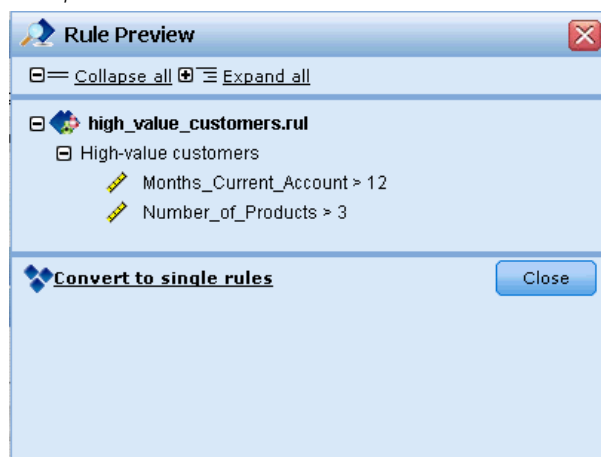
Figure 6-11 Rule preview
