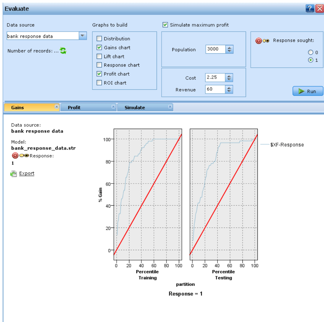
Figure 7-16 Simulation settings
