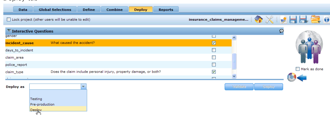
Figure 10-1 Deploy tab
