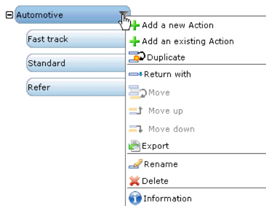
Figure 8-2 Dimension tree
