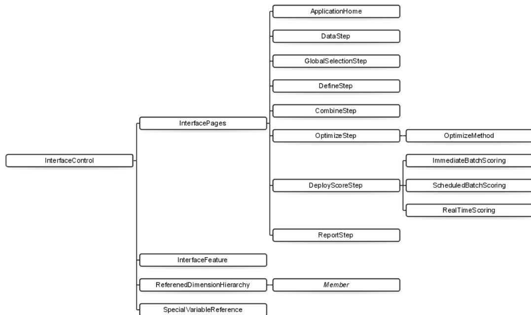
Abbildung 2-2 Element "InterfaceControl"
