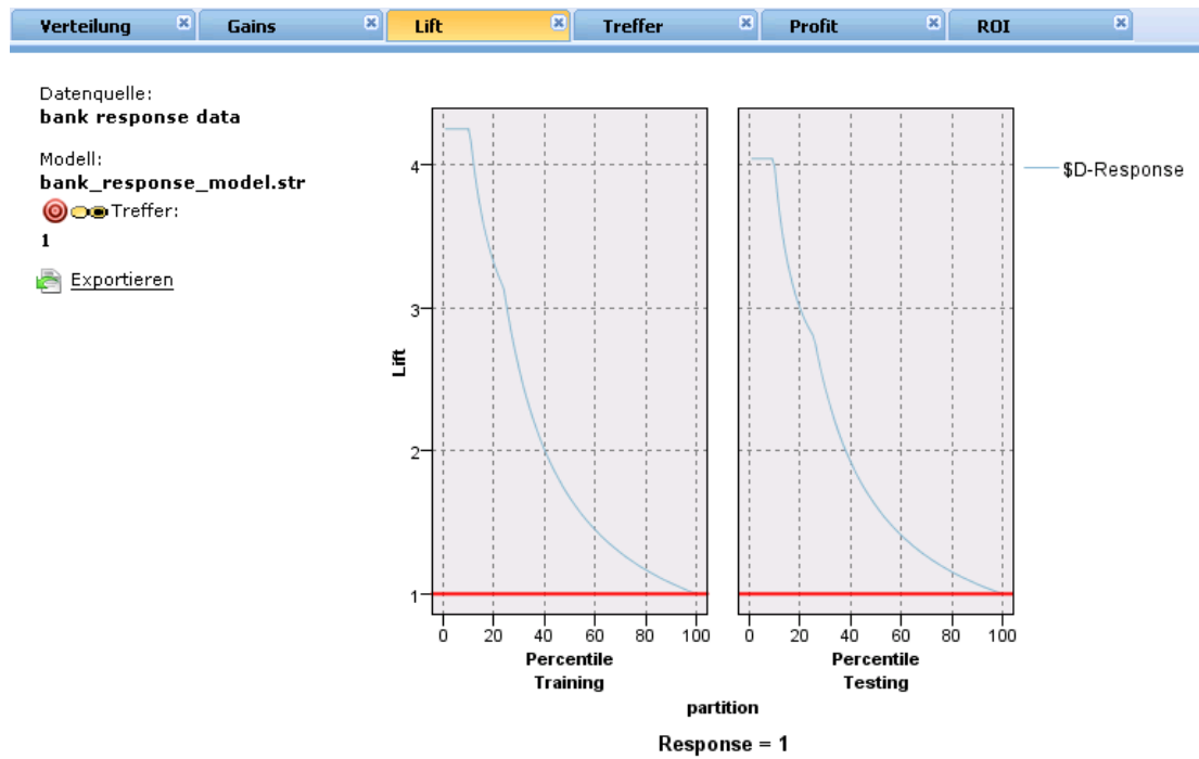
Abbildung 5-4 Lift Chart (Index)
