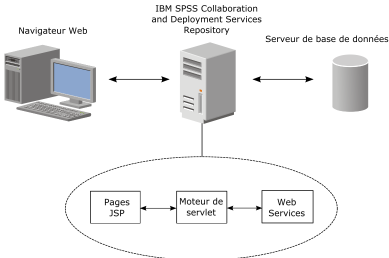
Figure 1. Architecture JSP
