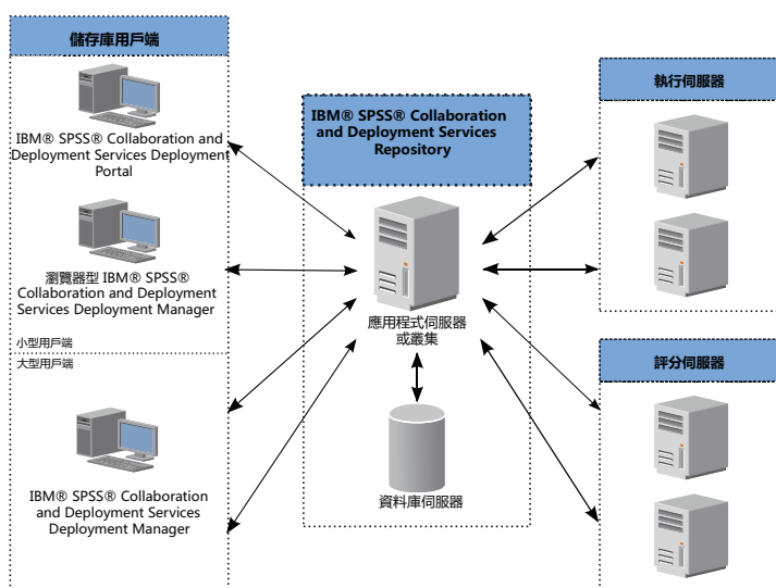
圖 1. IBM SPSS Collaboration and Deployment Services 架構
