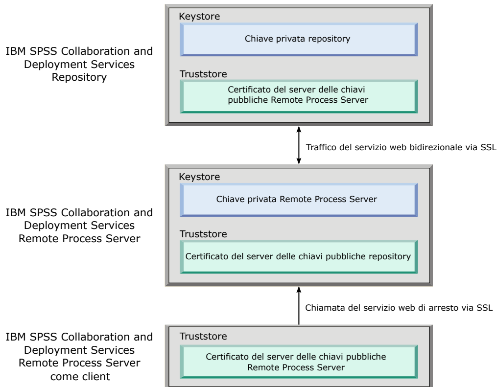
Figura 1. Architettura SSL per IBM SPSS Collaboration and Deployment Services Remote Process Server
