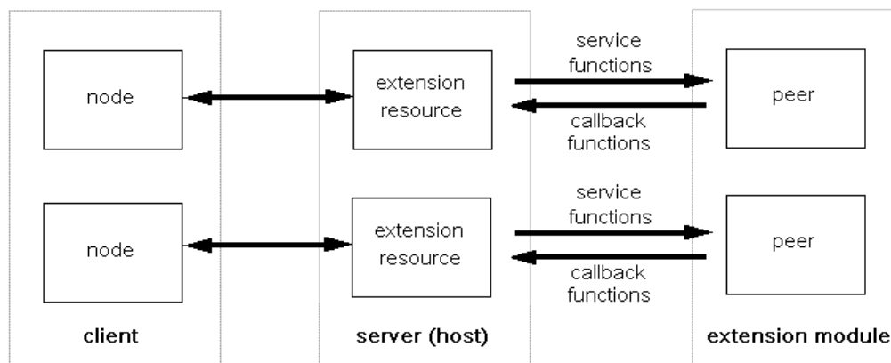
Figure 9-1 CLEF API architecture
