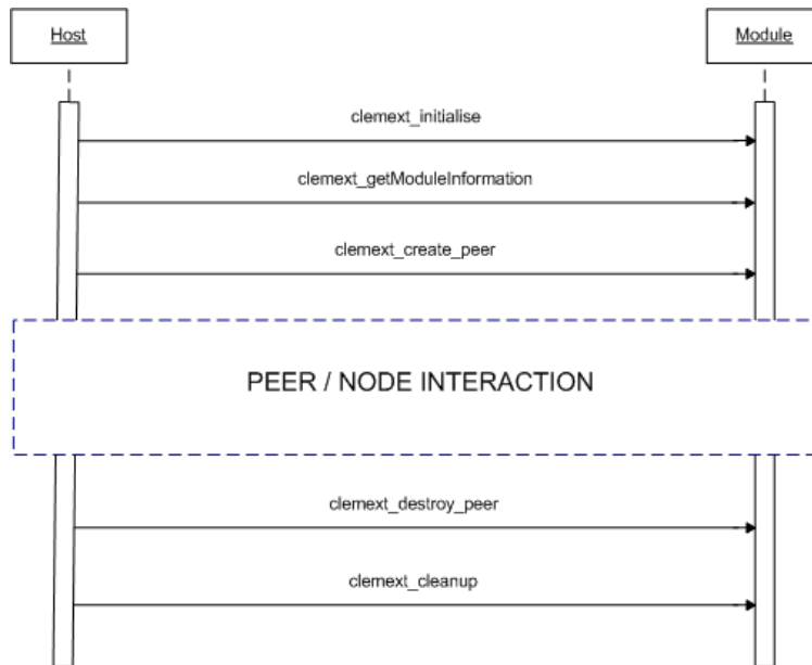
Figure 9-2 Typical process flow
