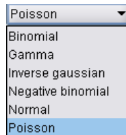
Figure 6-21 Combo box
