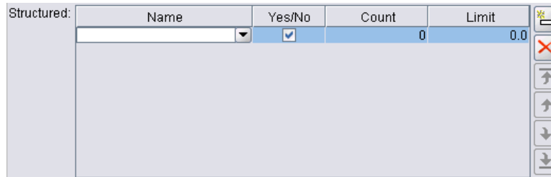
Figure 6-38 Table control
