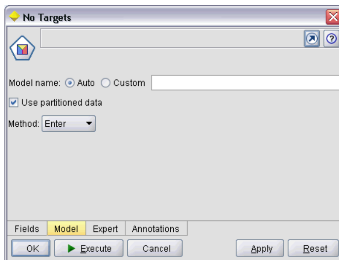
Figure 6-1 Tabbed dialog
