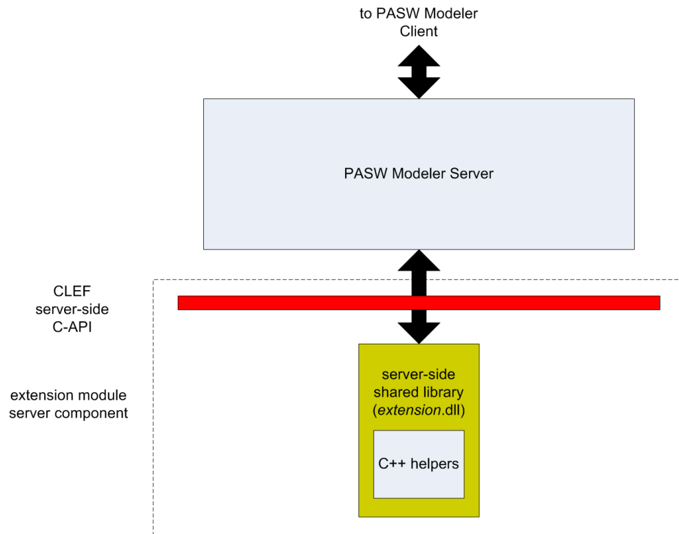
Figure 1-2 Server-side components
