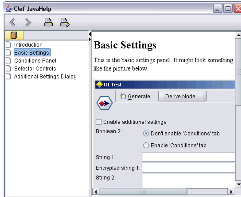
Figure 7-2 JavaHelp browser
