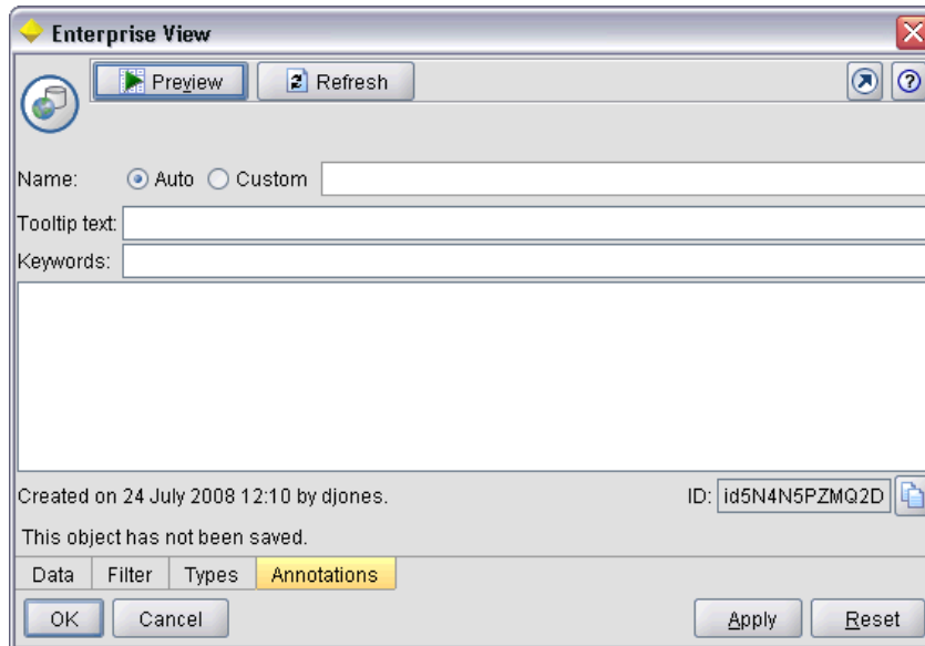
Figure 2-18 Annotations tab
