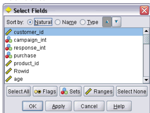
Figure 6-27 Multi-field list
