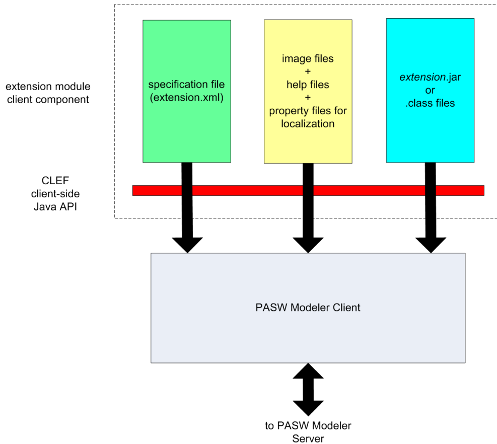
Figure 1-1 Client-side components
