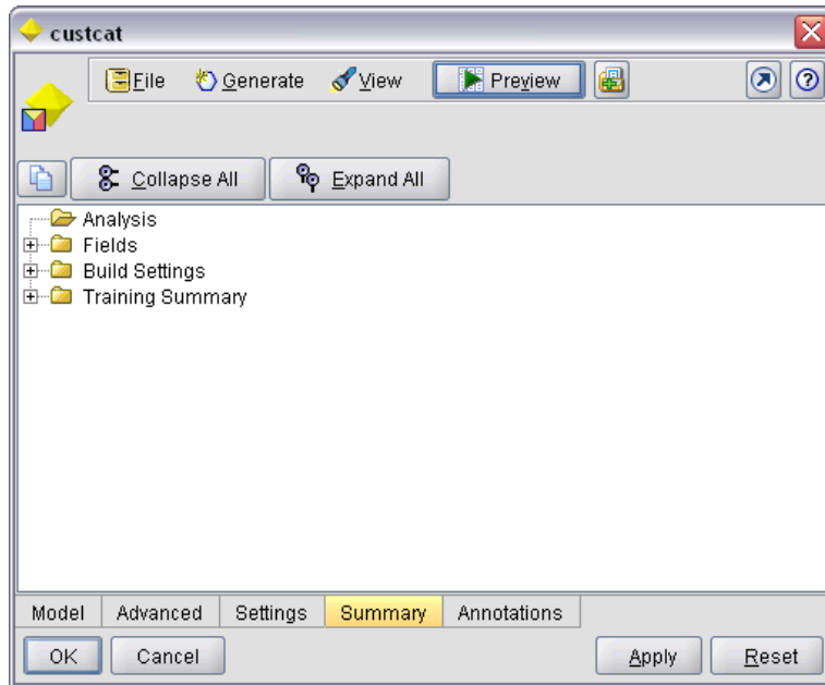
Figure 2-17 Summary tab
