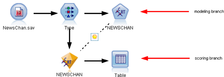
Figure 5-28 Modeling and scoring branches in a stream
