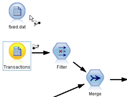
Figure 5-40 Selecting a replacement source node
