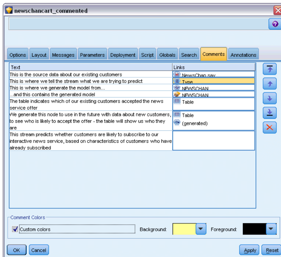
Figure 5-34 Listing comments for a stream
