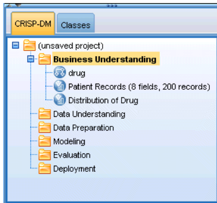
Figure 11-2 CRISP-DM view
