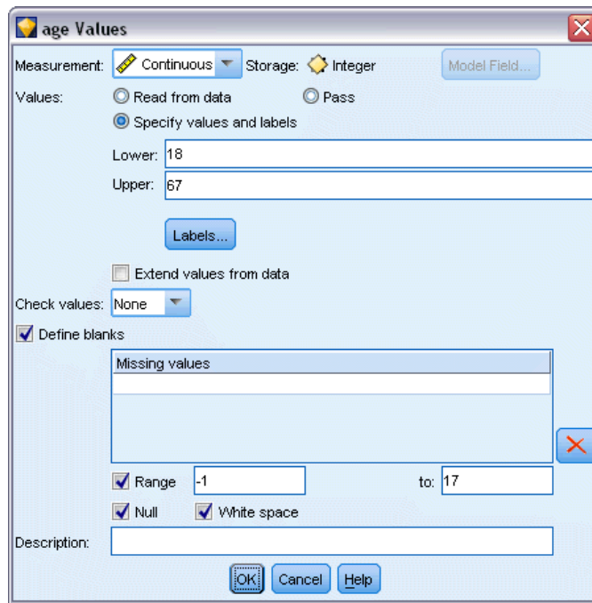
Figure 6-1 Specifying missing values for a continuous variable
