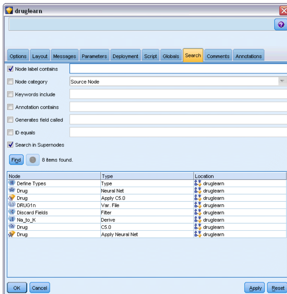
Figure 5-24 Searching for nodes in a stream
