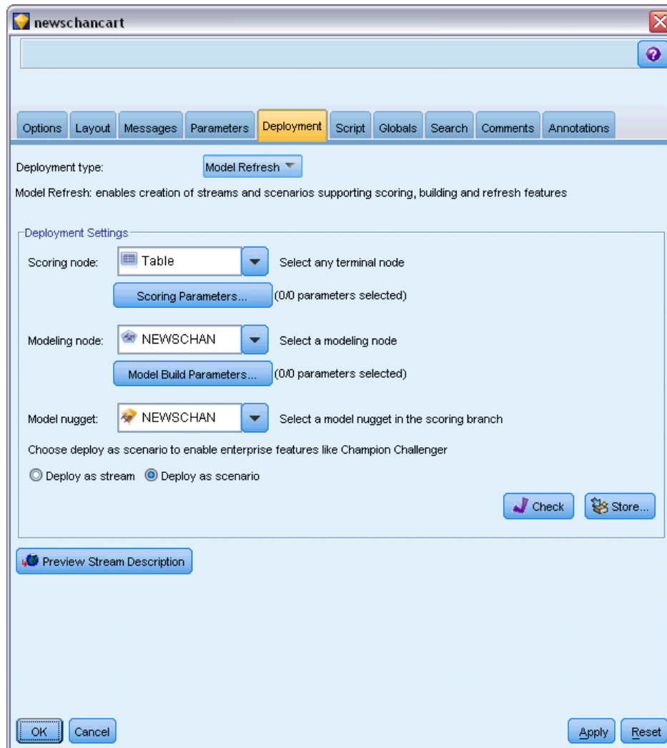
Figure 9-24 Stream Deployment options
