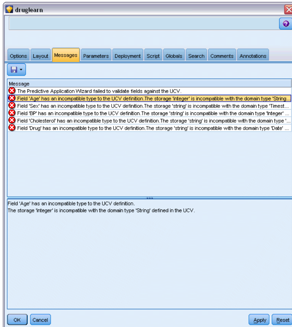
Figure 10-7 Error messages resulting from metadata mismatch
