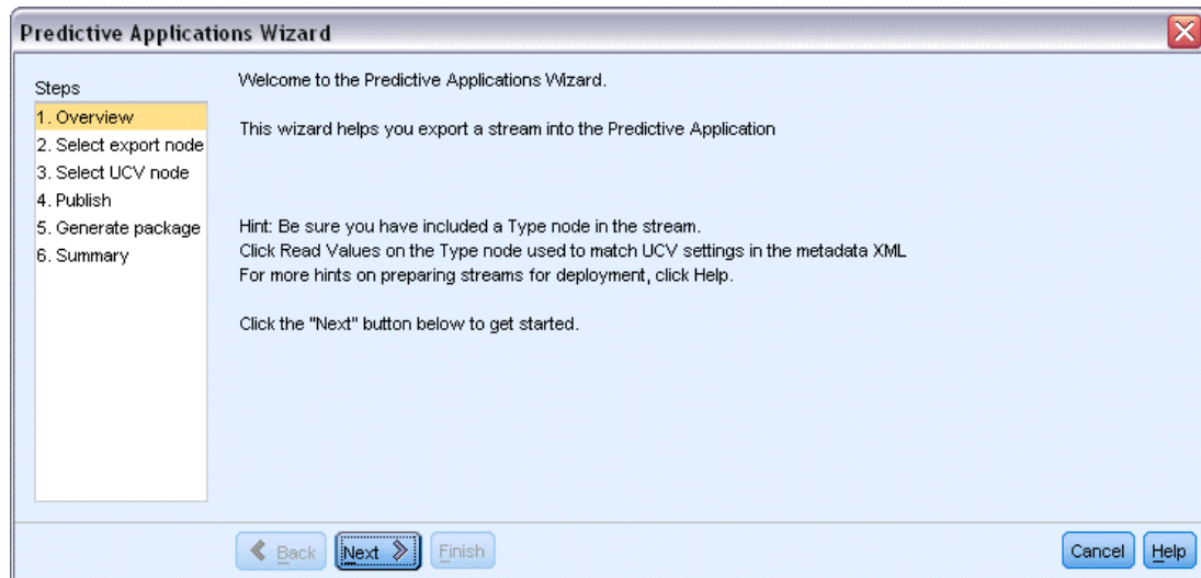
Figure 10-1 Predictive Applications Wizard
