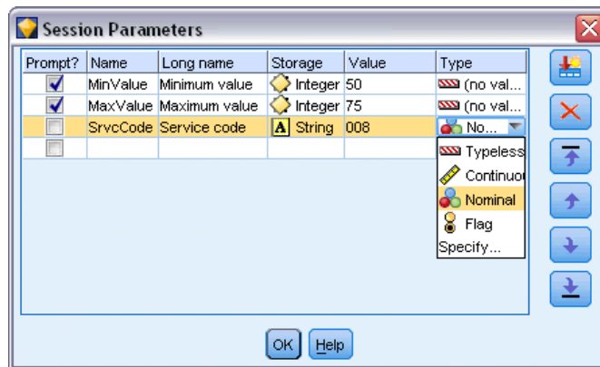
Figure 5-20 Setting parameters for the session
