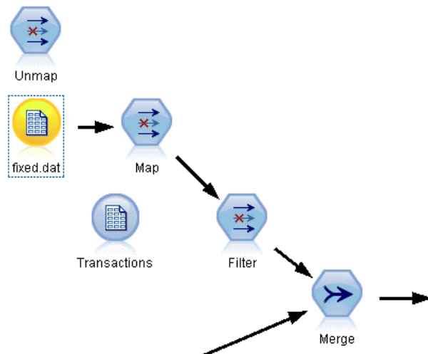
Figure 5-41 New data source successfully mapped to the stream
