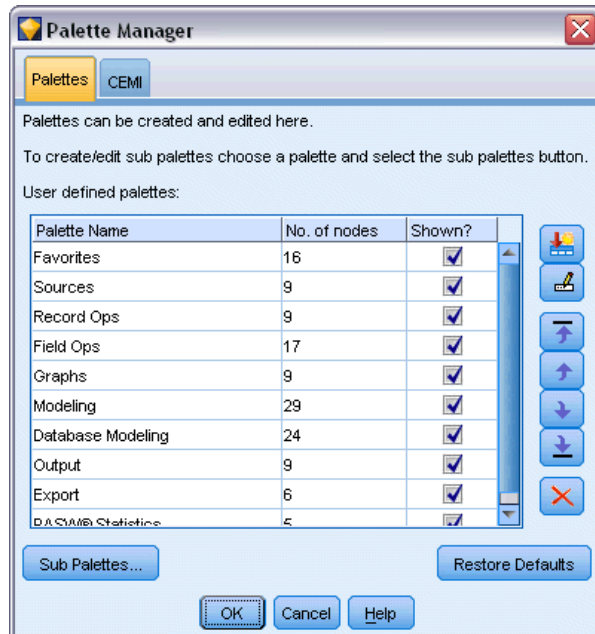
Figure 5-45 Palette Manager
