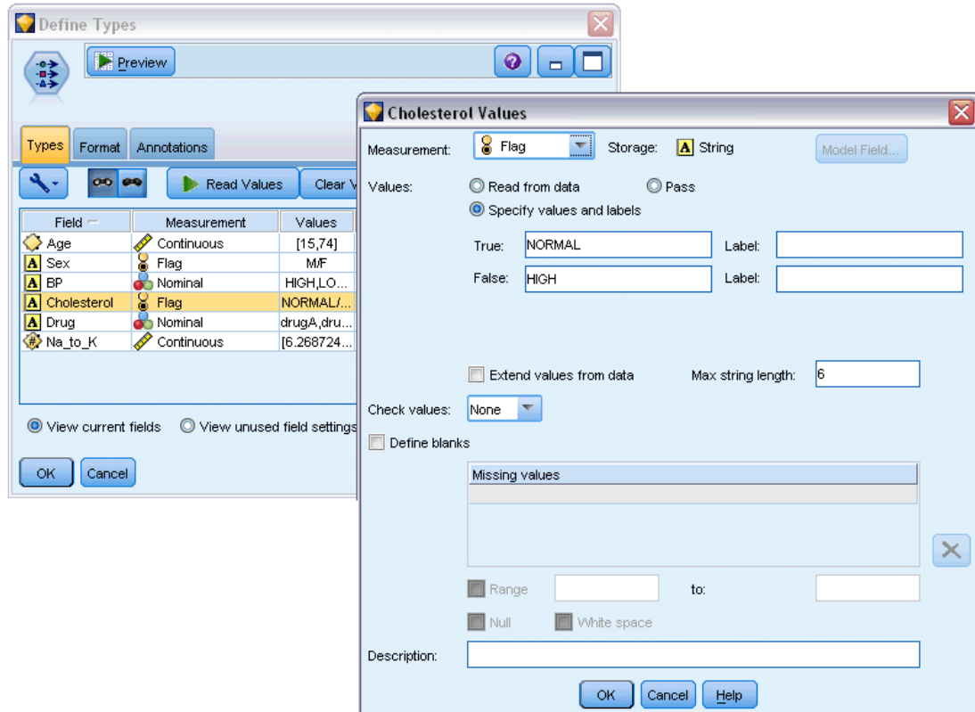
Figure 10-4 Checking Type node settings and storage in the Values subdialog box
