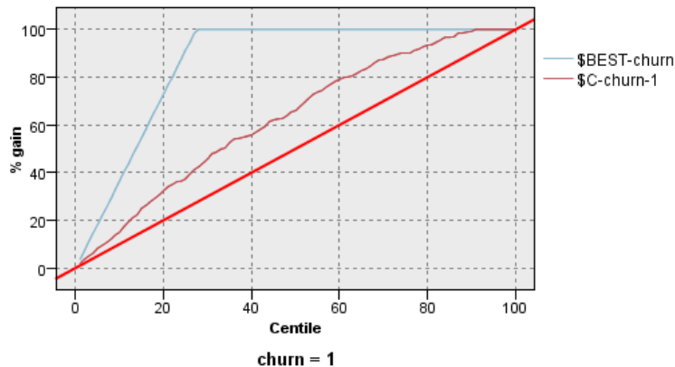
Figure 27-18 Graphiques de gains
