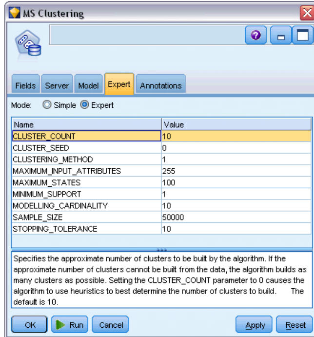
Figure 3-8 Classification MS - Options expert
