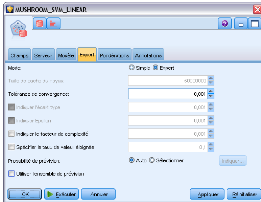
Figure 4-11 Options expert SVM
