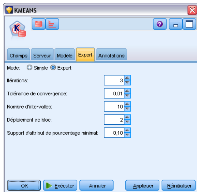
Figure 4-21 Options expert de k-Means
