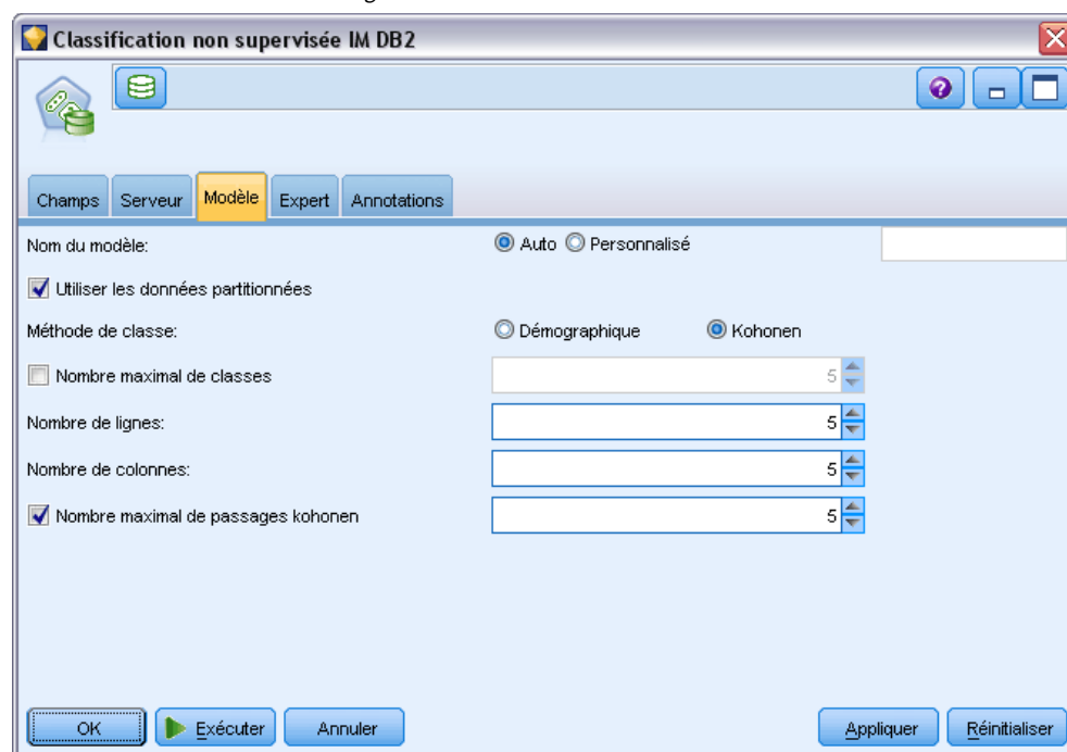
Figure 5-24 Noeud Classification ISW - Onglet Modèle
