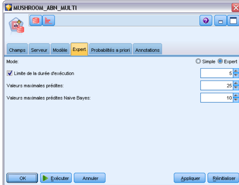
Figure 4-9 Options expert Adaptive Bayes
