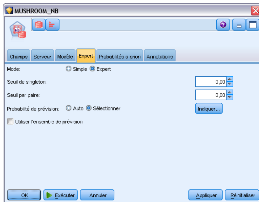
Figure 4-7 Options expert Naive Bayes
