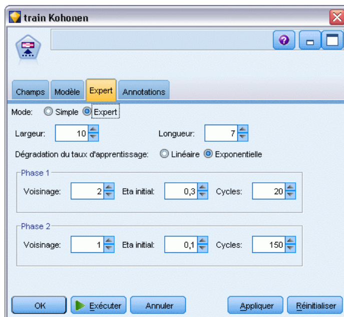
Figure 11-5 Kohonen - Options expert
