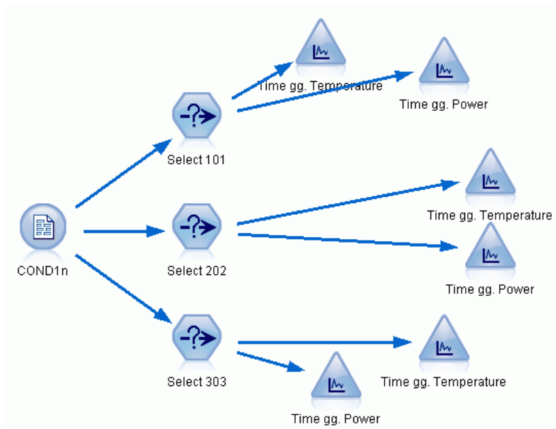
Abbildung 20-1 Condplot-Stream
