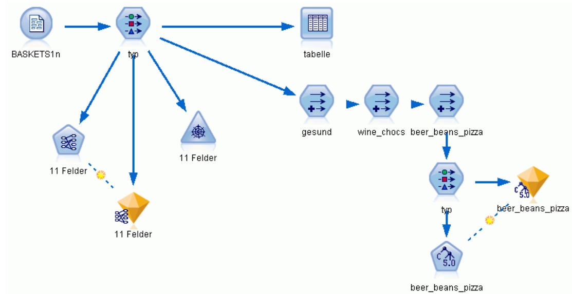
Abbildung 27-1 baskrule-Stream
