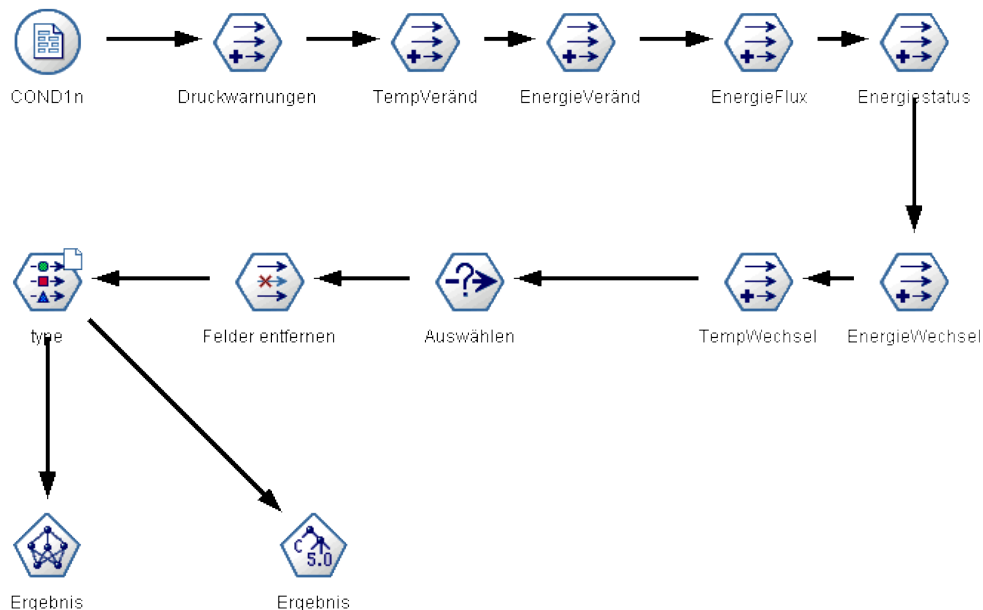
Abbildung 20-3 Condlearn-Stream
