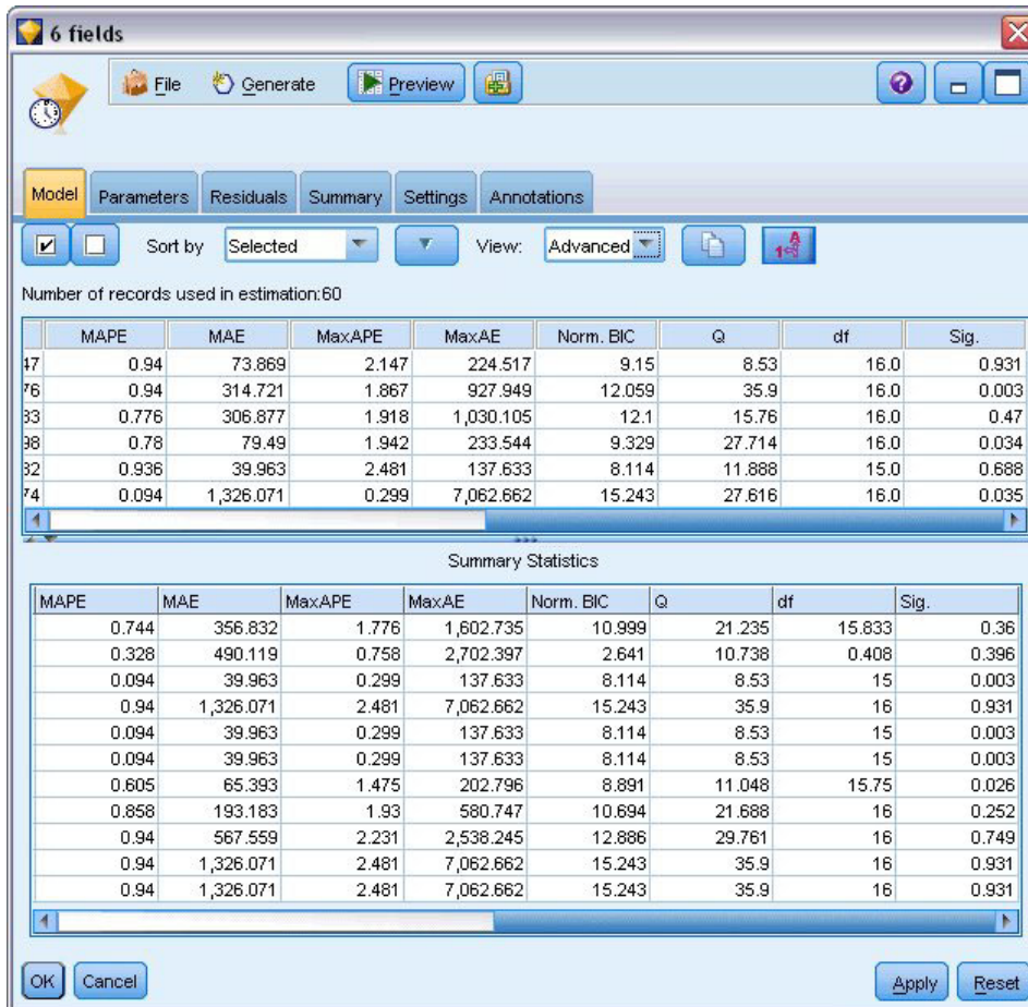
Figure 185. Time Series models advanced display
