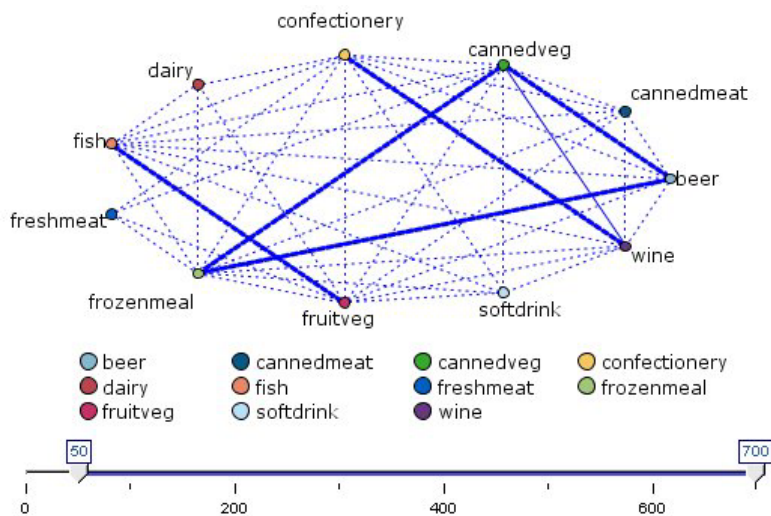
Figure 37. Web graph showing relationships between the purchase of grocery items
