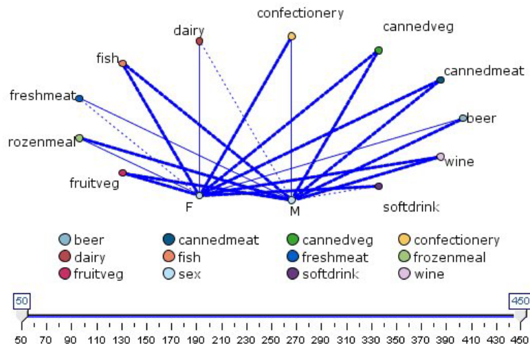
Figure 38. Directed web graph showing the relationship between the purchase of grocery items and gender
