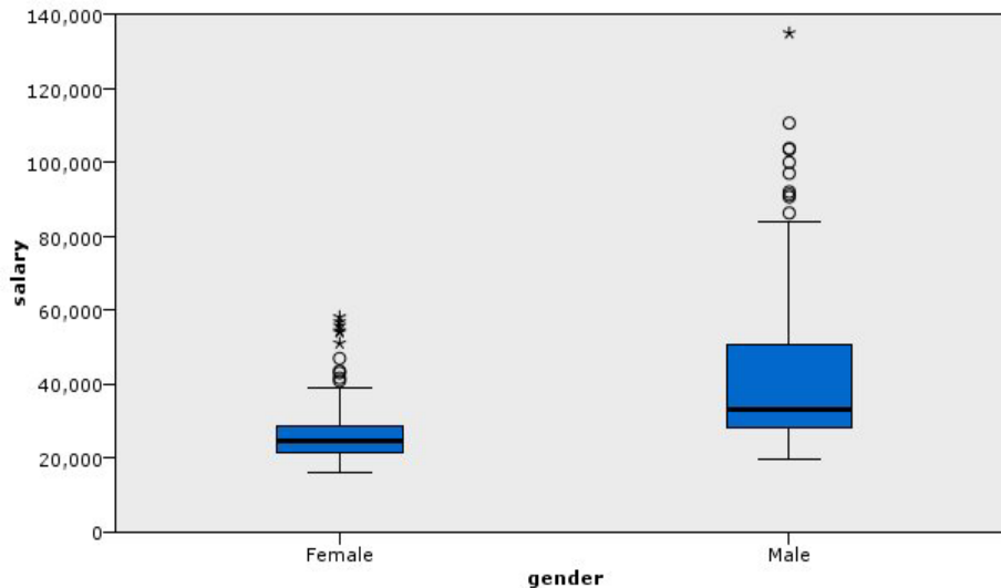
Figure 14. Boxplot
