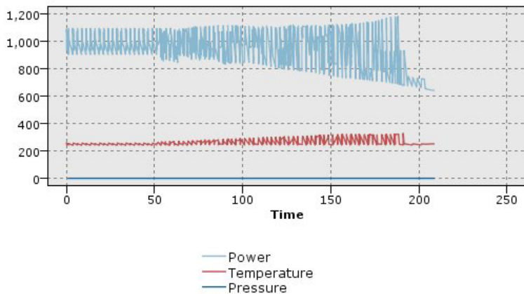
Figure 26. Standard multiplot showing power-plant fluctuation over time (note that without normalizing, the plot for Pressure is impossible to see)
