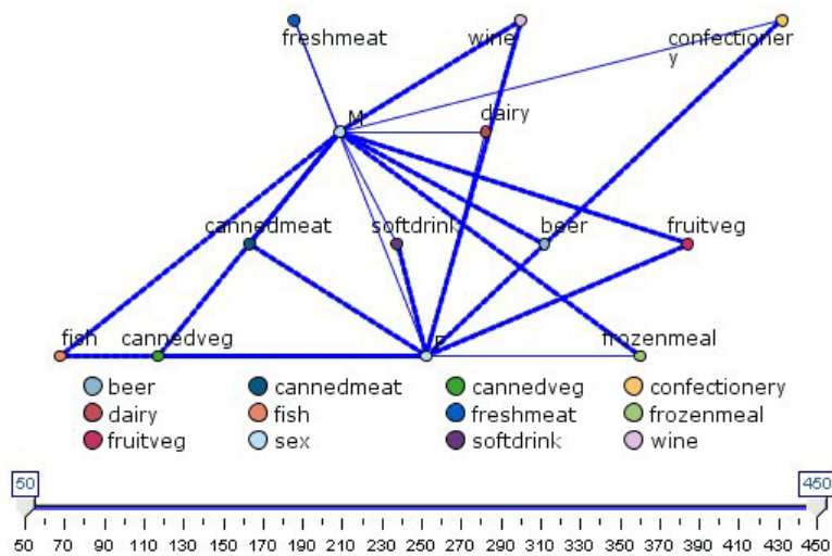
Figure 39. Web graph showing strong connections from frozenmeal and cannedveg to other grocery items
