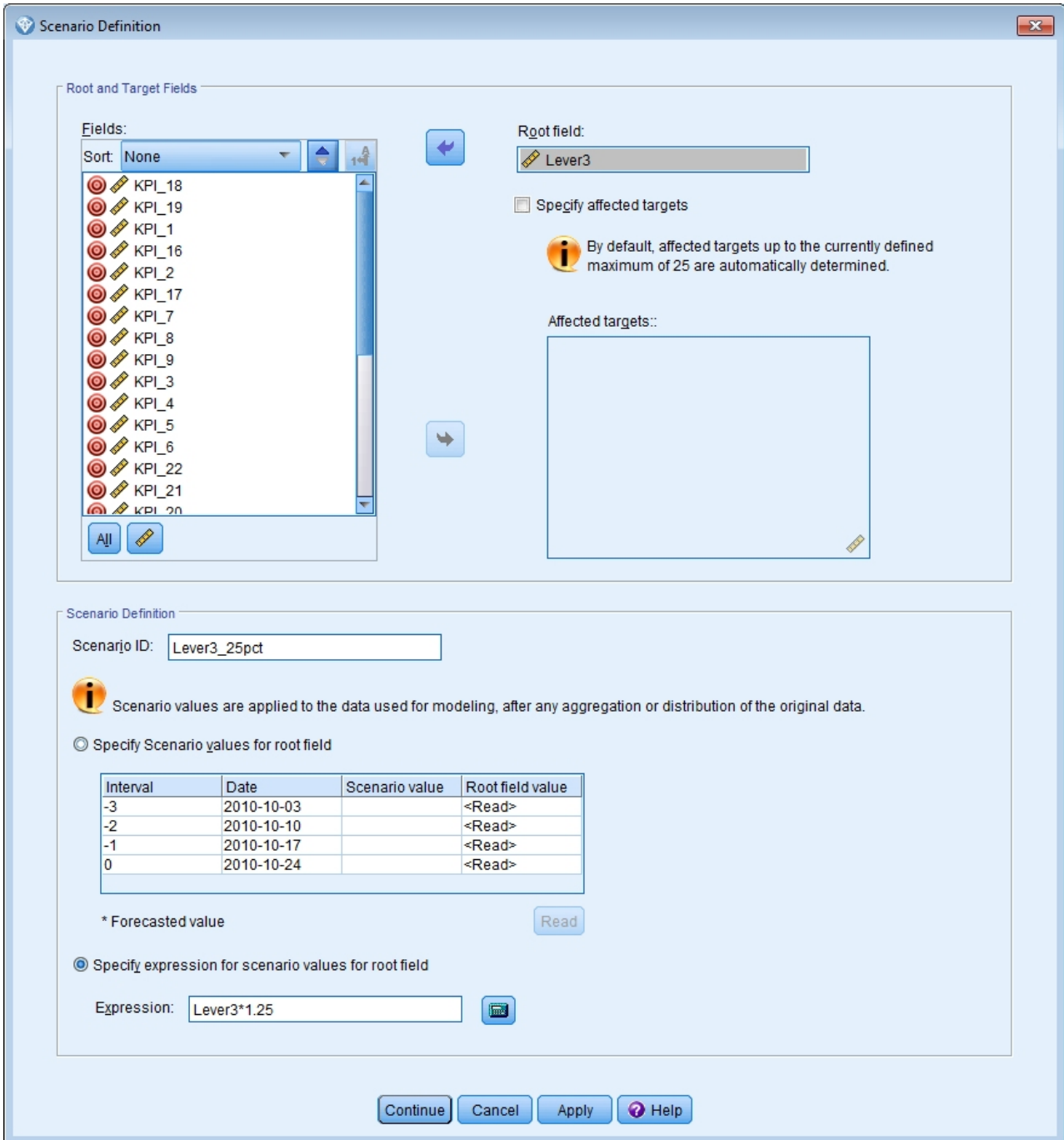
Figure 414. Scenario Definition
