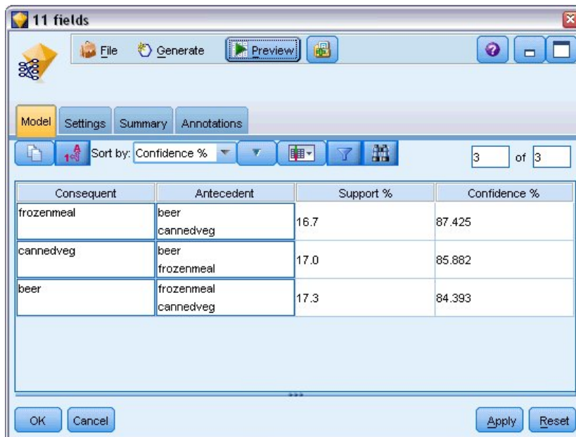
Figure 386. Association rules
