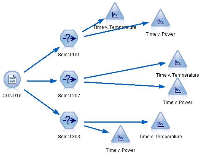
Figure 263. Condplot stream
