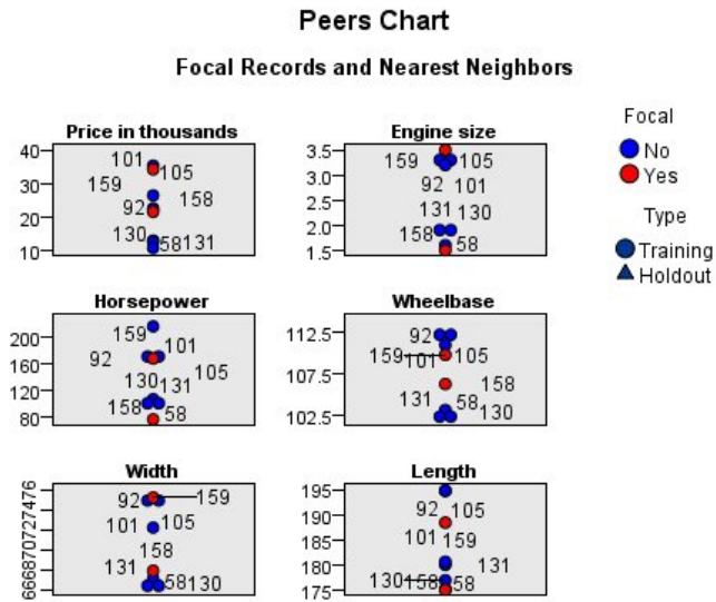
Figure 397. Peers chart
