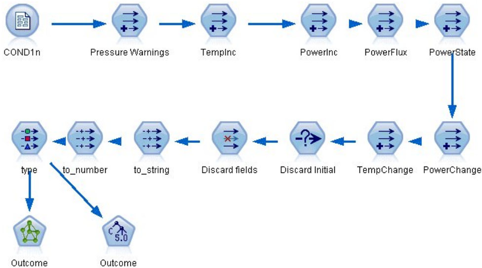
Figure 265. Condlearn stream
