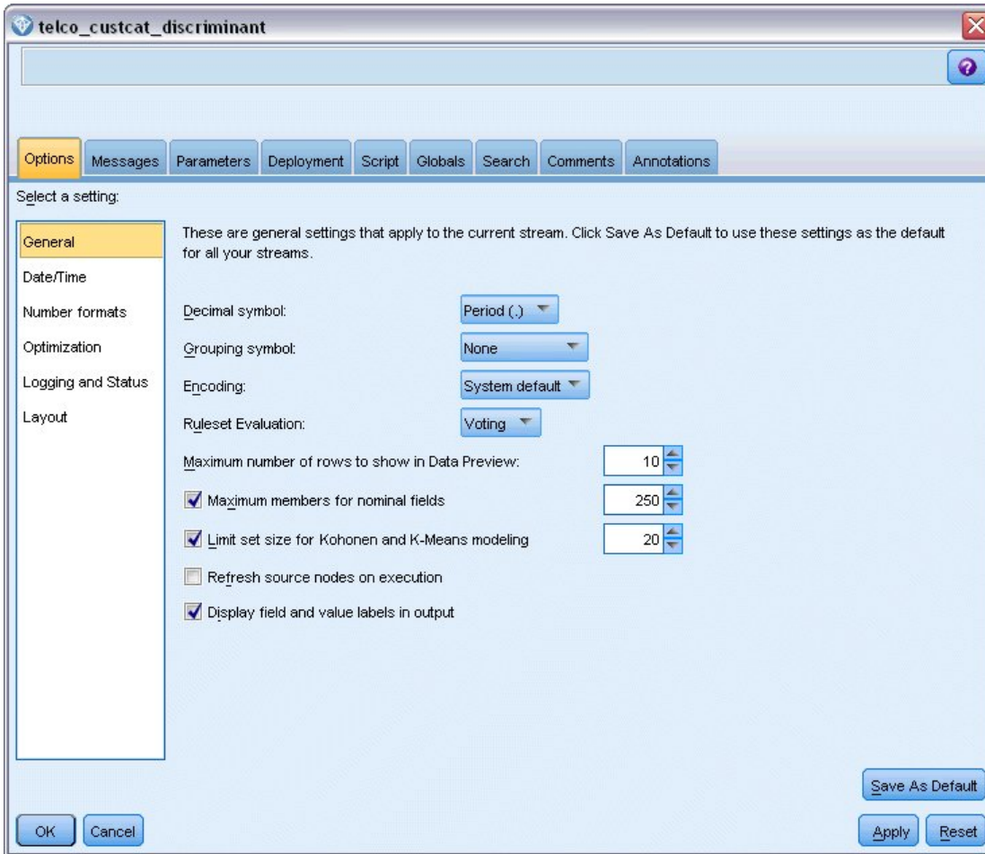
Figure 268. Stream properties
