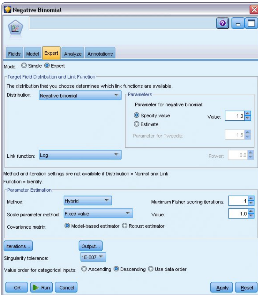
Figure 323. Expert tab
