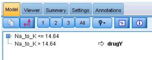
Figure 97. Rule browser
