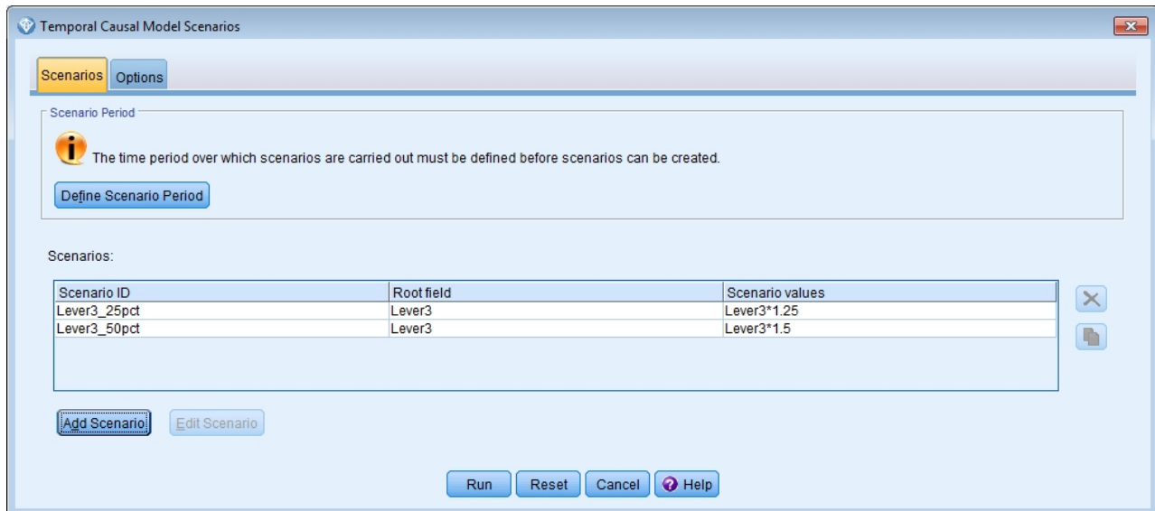
Figure 415. Scenarios
