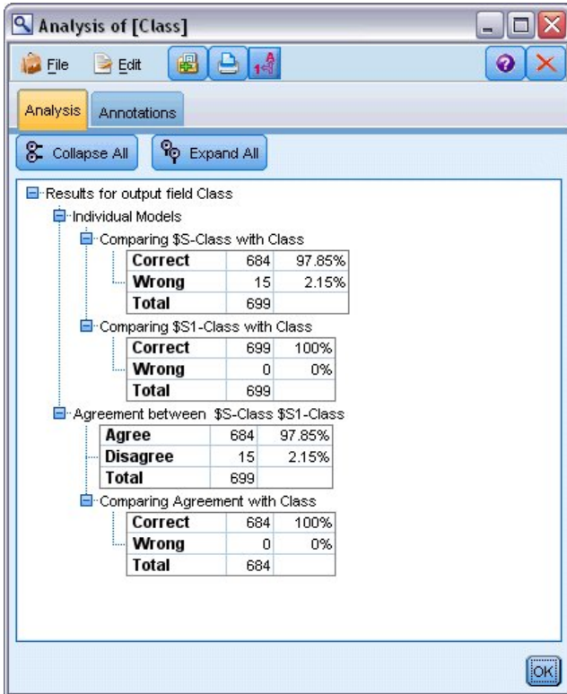
Figure 342. Analysis node
