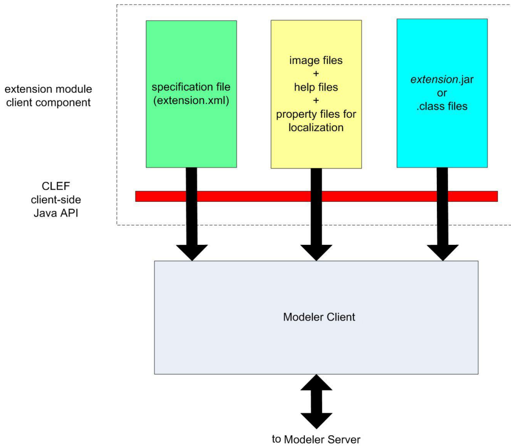
Figure 1. Client-side components
