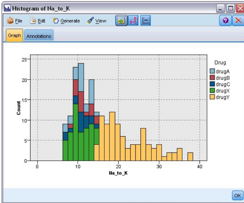
Figure 2. Sample histogram
