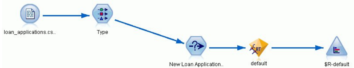
Figure 7. Stream selecting new loan applications and with Distribution node added
