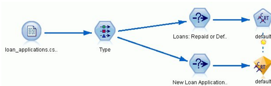
Figure 6. Stream with model nugget added
