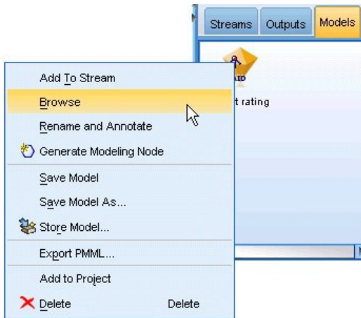
Figure 8. Models palette
