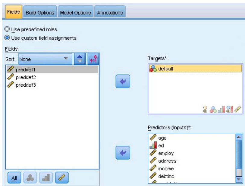
Figure 30. Fields tab
