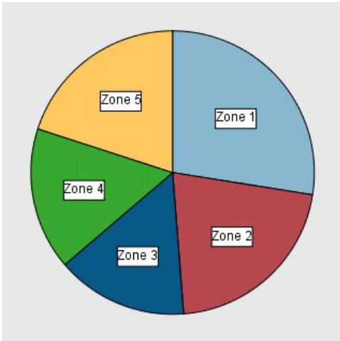
Figure 15. Pie chart
