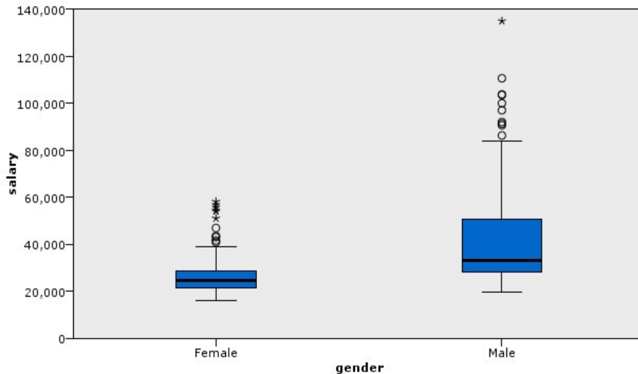
Figure 14. Boxplot
