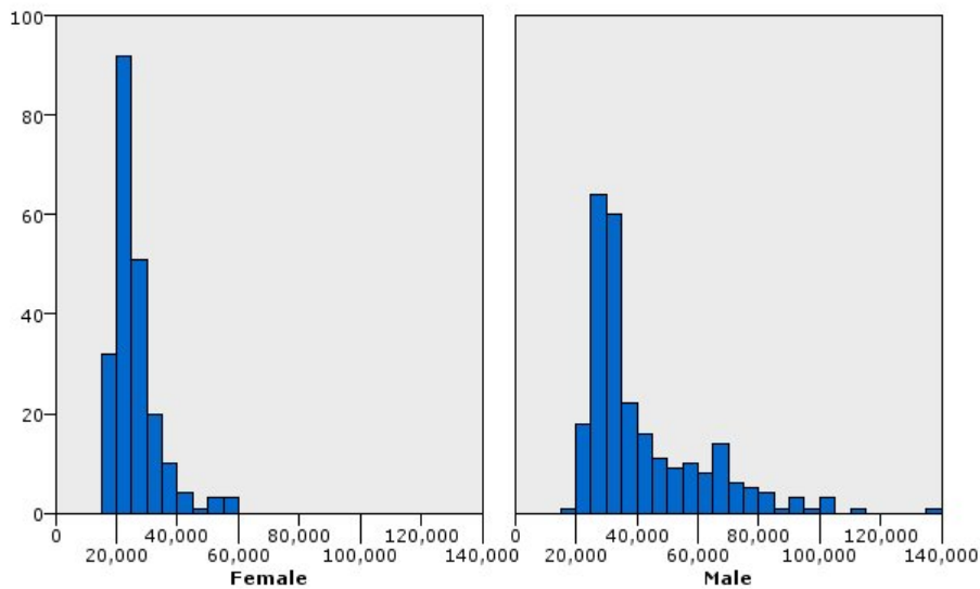
Figure 12. Paneled histogram
