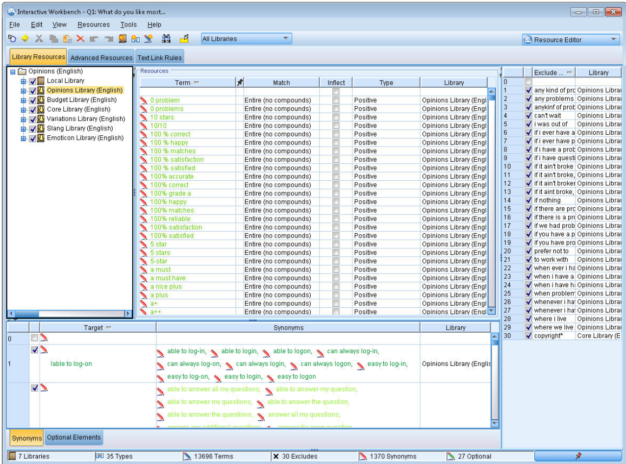
Figure 35. Resource Editor view for Non-Japanese Languages
