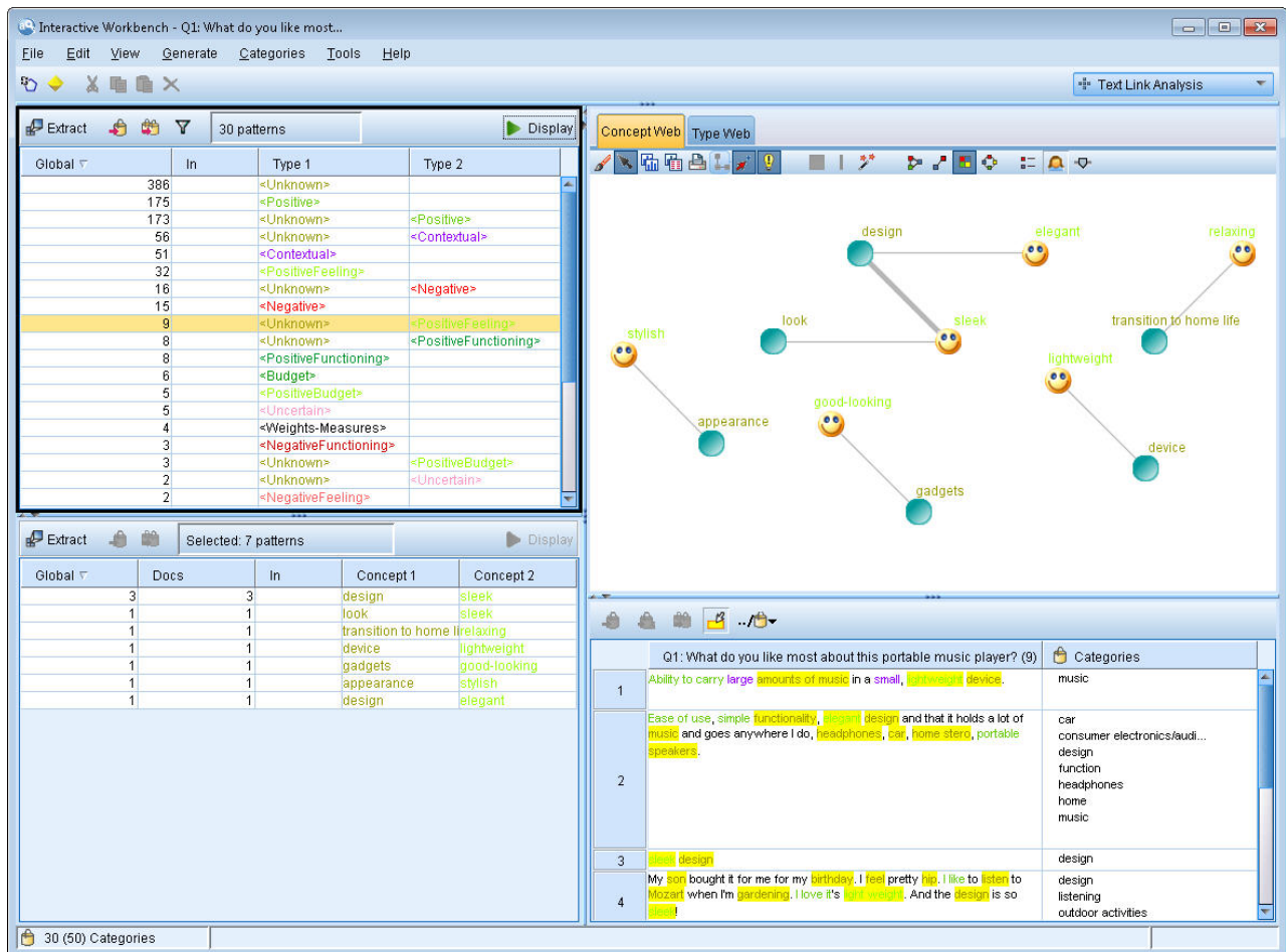
Figure 25. Text Link Analysis view
