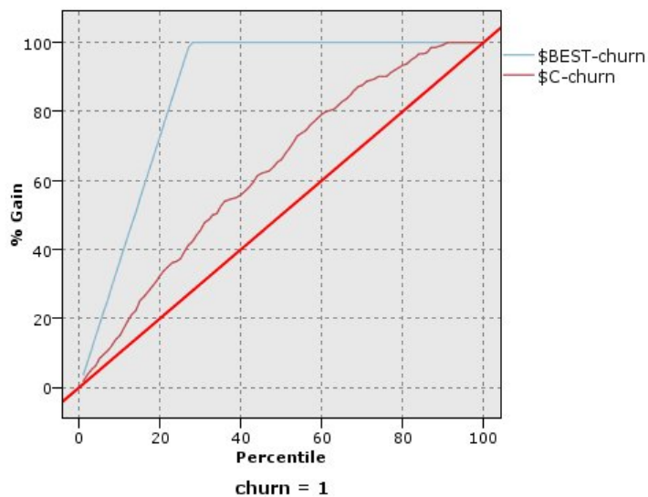
Figure 357. Gains chart
