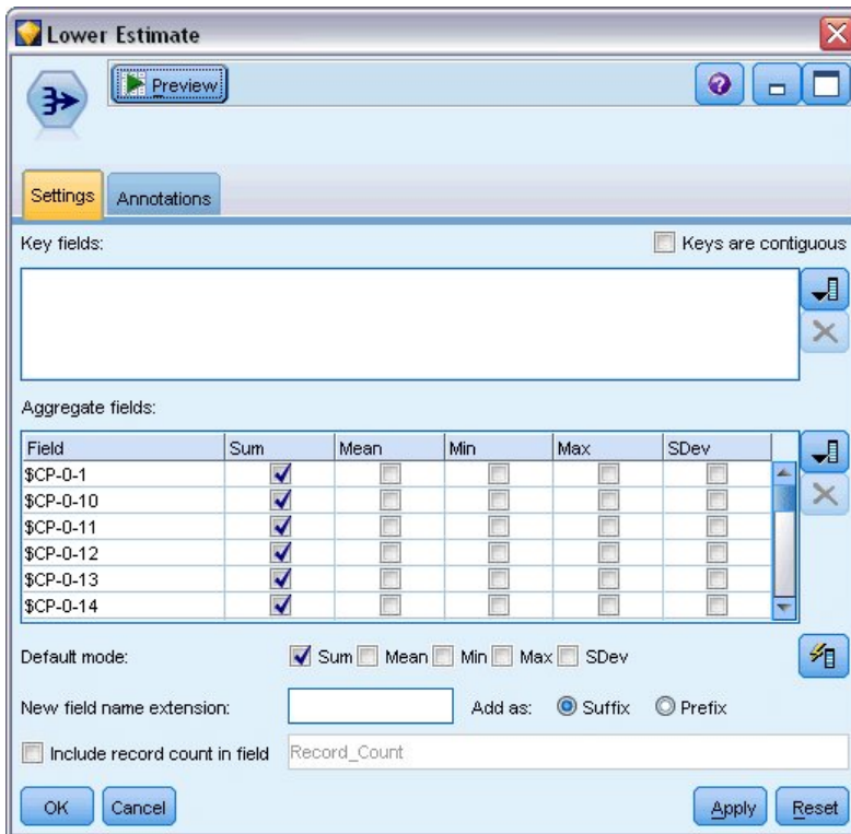
Figure 361. Aggregate node: Settings tab
