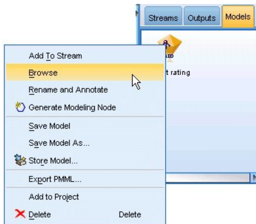
Figure 18. Models palette
