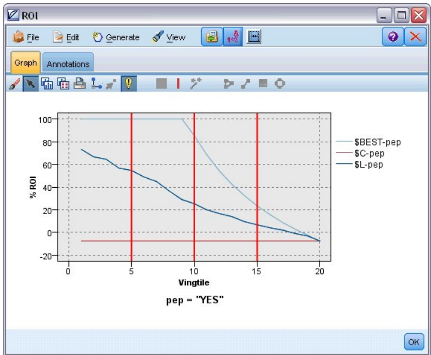
Figure 59. Graph with three bands
