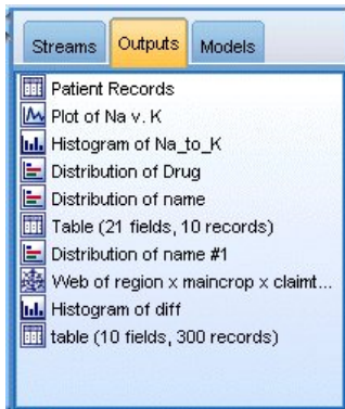
Figure 6. Outputs tab
