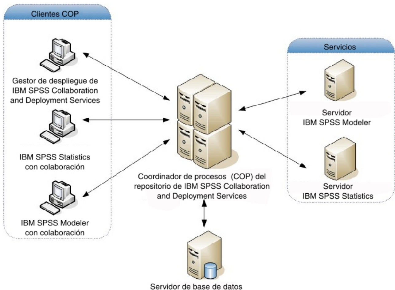
Figura 5. Arquitectura de Coordinator of Processes
