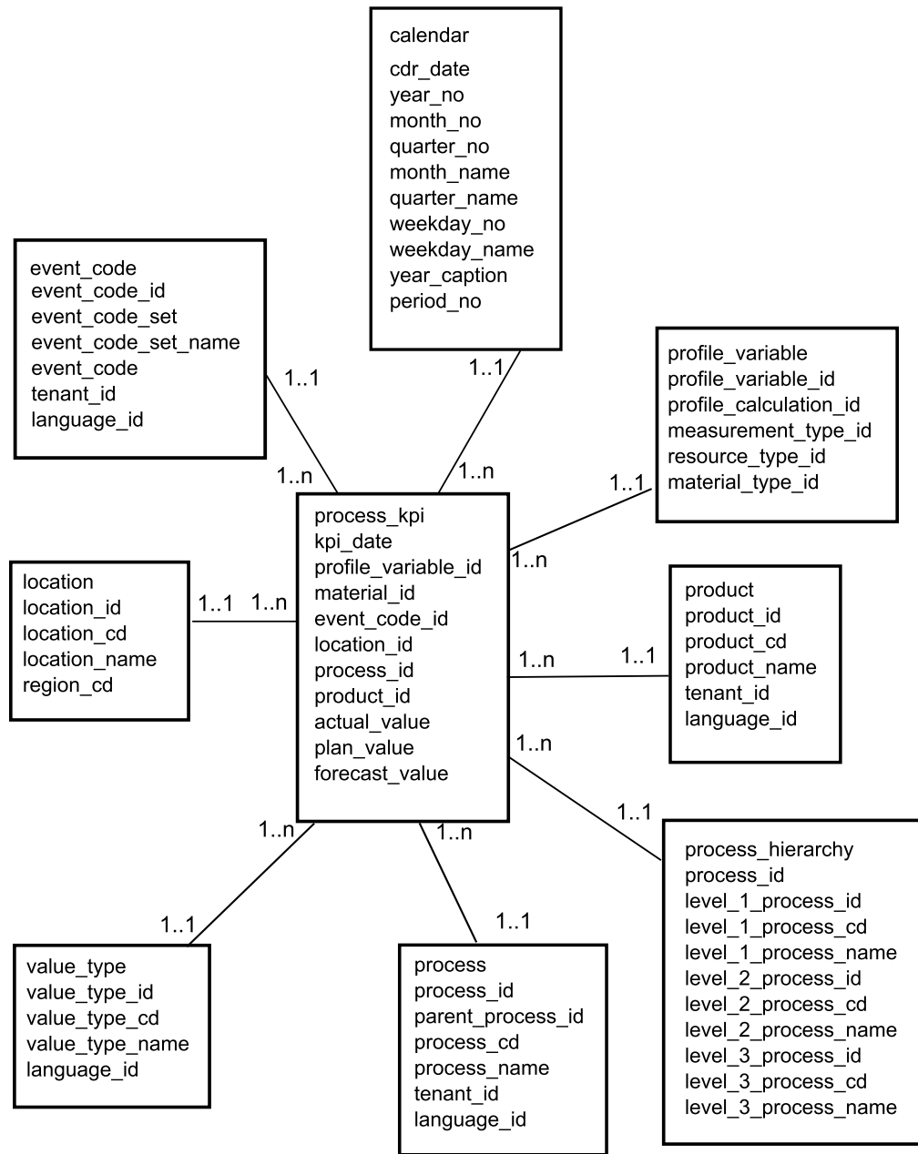
Figure 14. The process_kpi star schema
