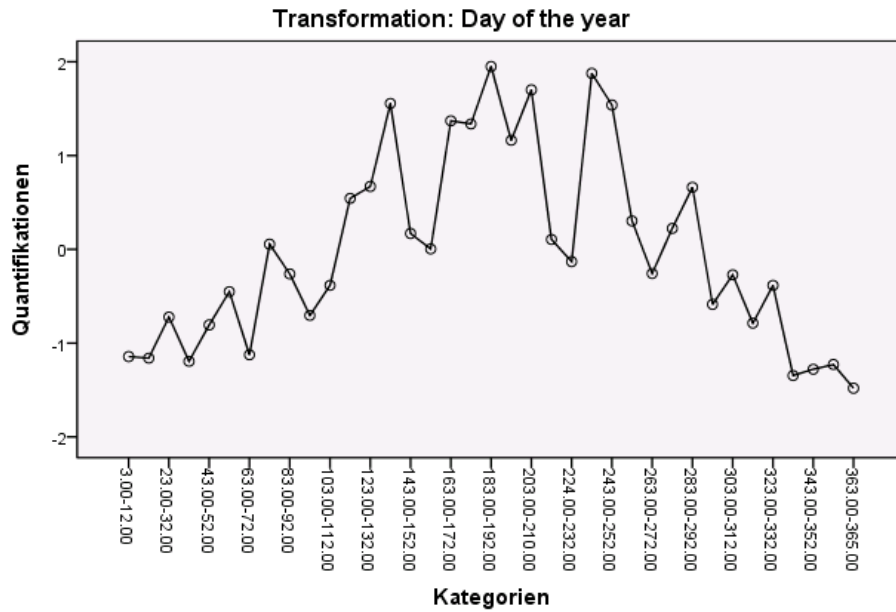
Abbildung 9-55 Transformationsdiagramm von "Day of the year" (nominal)
