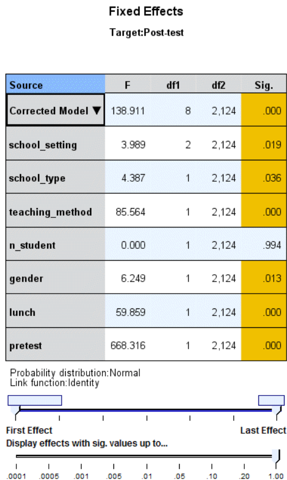
Figure 8-17 Fixed Effects view, table style
