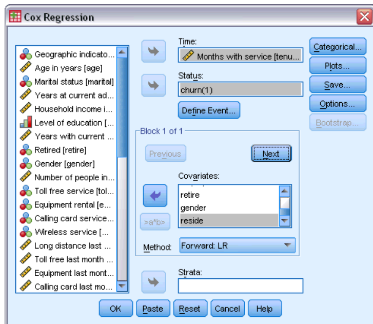
Figure 14-1 Cox Regression dialog box
