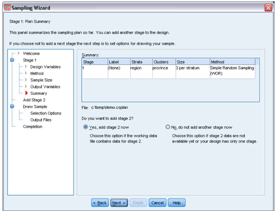
Figure 13-17 Sampling Wizard, Plan Summary step (stage 1)
