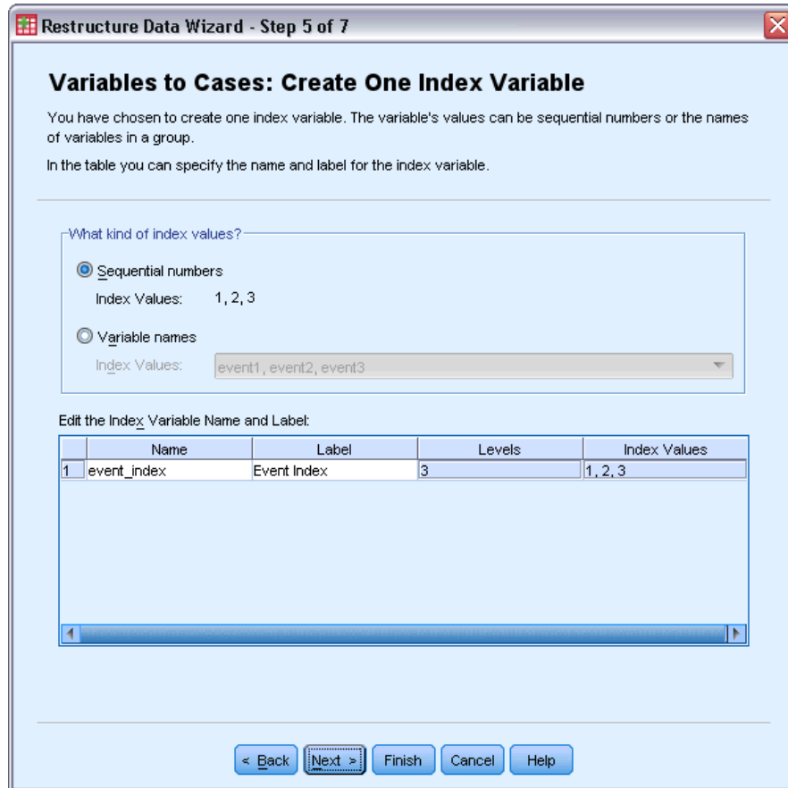
Figure 22-31 Restructure Data Wizard, Variables to Cases Create One Index Variable step
