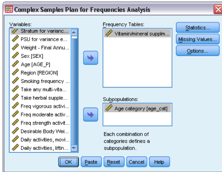
Figure 15-2 Frequencies dialog box
