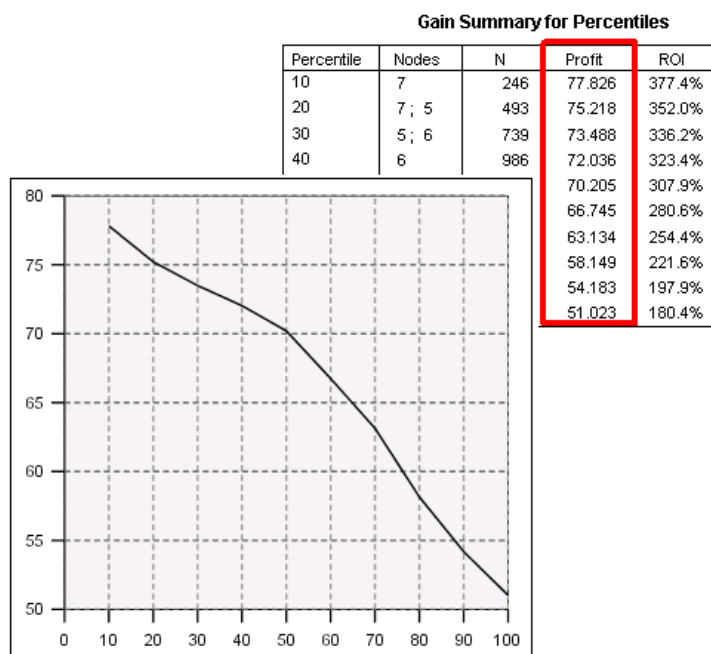
Figure 1-30 Gain summary for percentiles table and average profit chart
