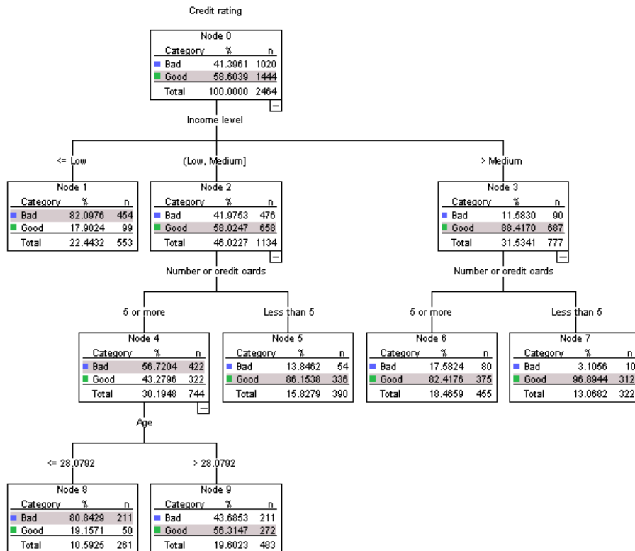
Figure 1-1 Decision tree
