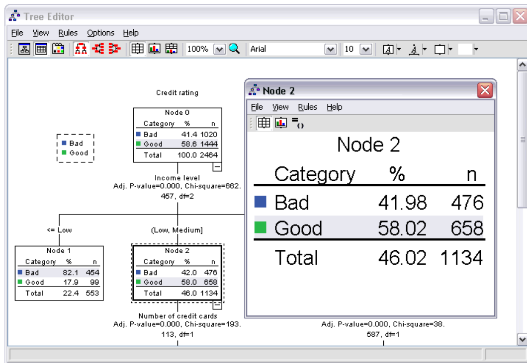
Figure 2-4 Summary window
