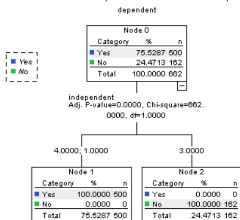
Figure 3-7 Tree for nominal dependent variable with partial value labels
