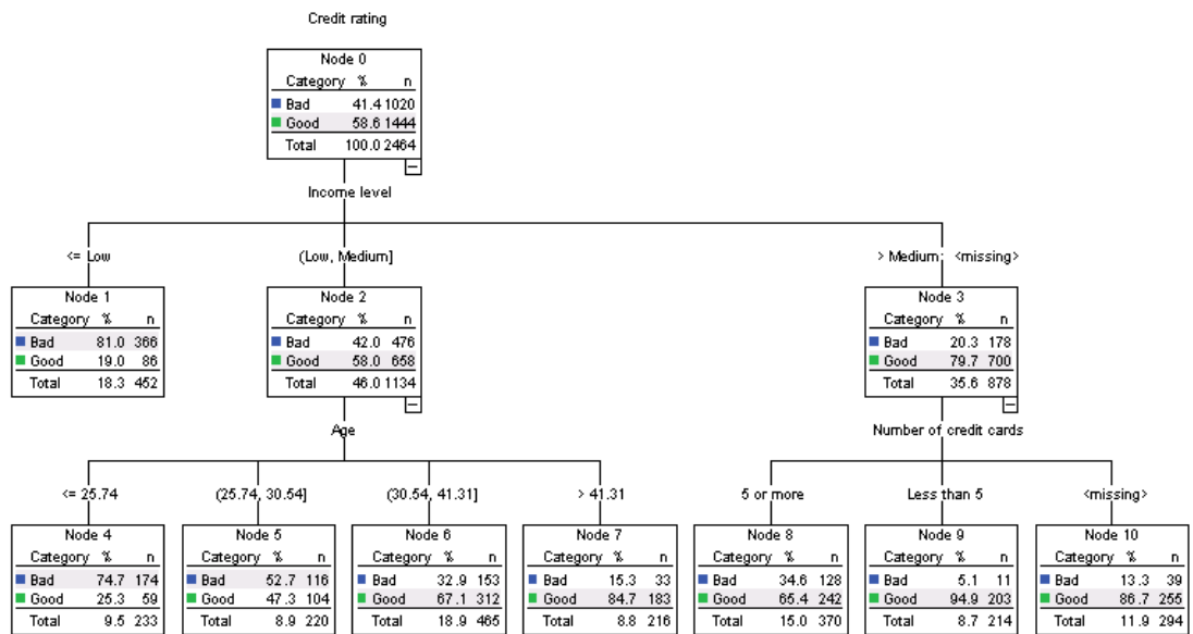
Figure 6-4 CHAID tree with missing independent variable values
