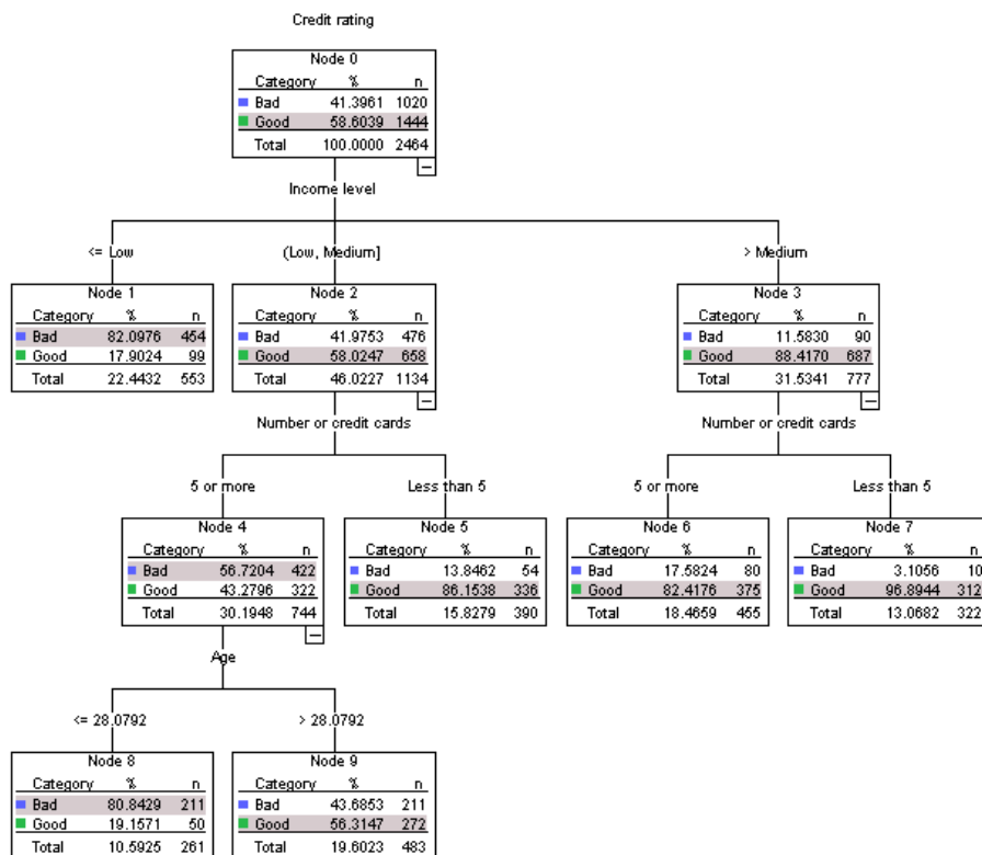
Figure 4-8 Tree diagram for credit rating model
