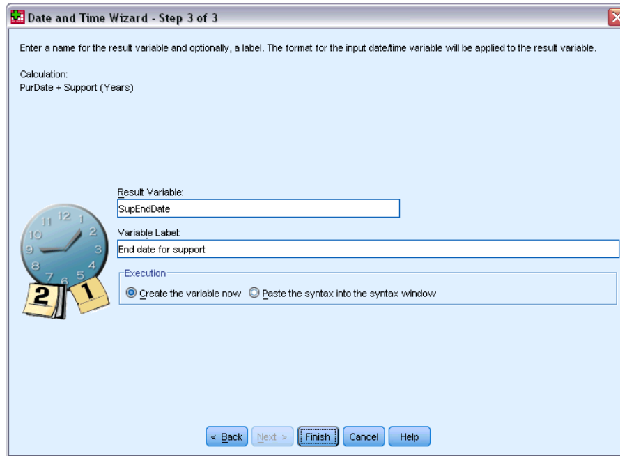
Figure 9-17 Adding a duration to a date: Step 3
