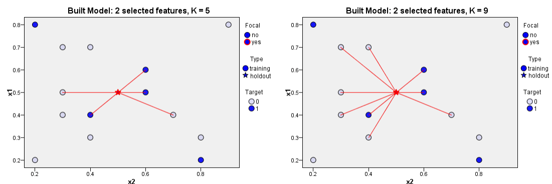
Figure 124-1 The effects of changing k on classification
