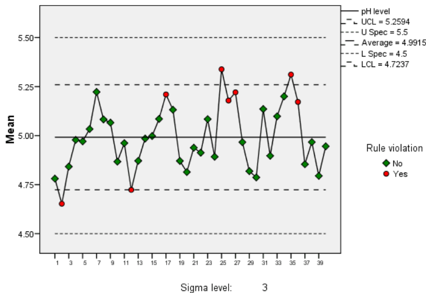
Figure 233-1 X-bar chart
