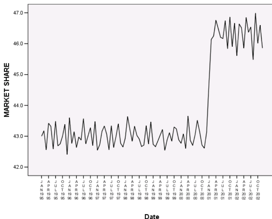
Figure 254-1 TSPLLOT VARIABLES=SHARE
