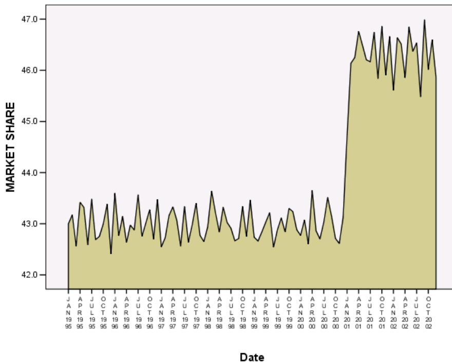
Figure 254-2 FORMAT=BOTTOM
