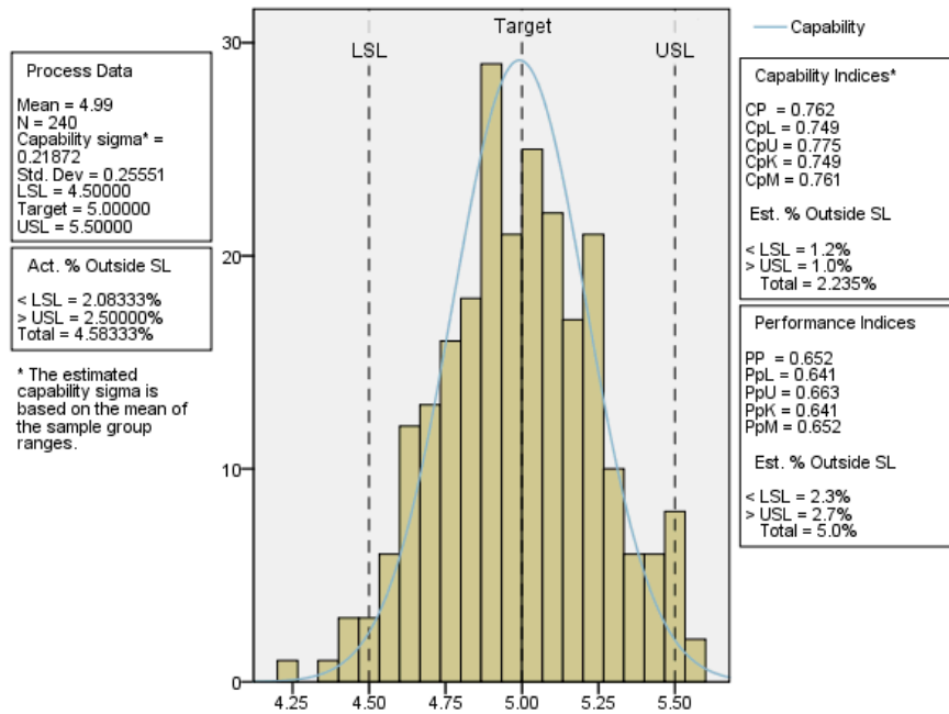
Figure 233-10 Process capability chart
