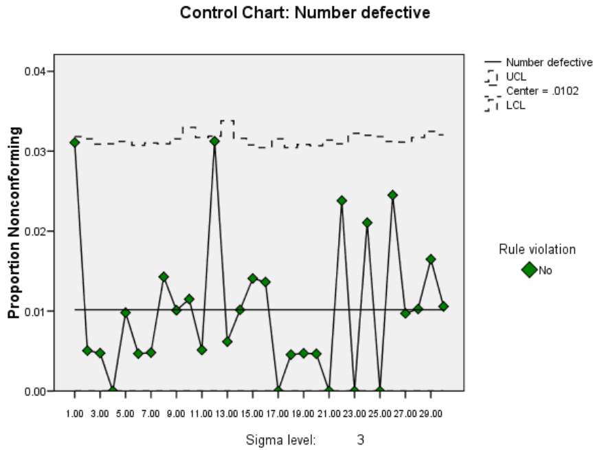
Figure 233-6 A p chart
