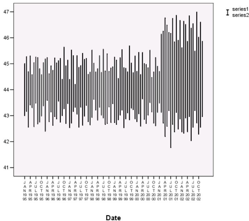
Figure 254-4 FORMAT=HILO
