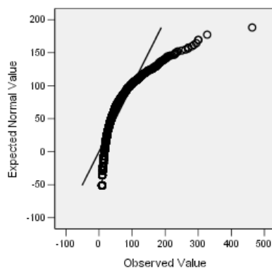
Figure 185-1 Normal q-q plot of household income
