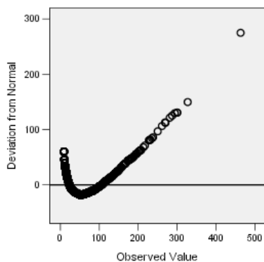
Figure 185-3 Detrended normal q-q plot of household income
