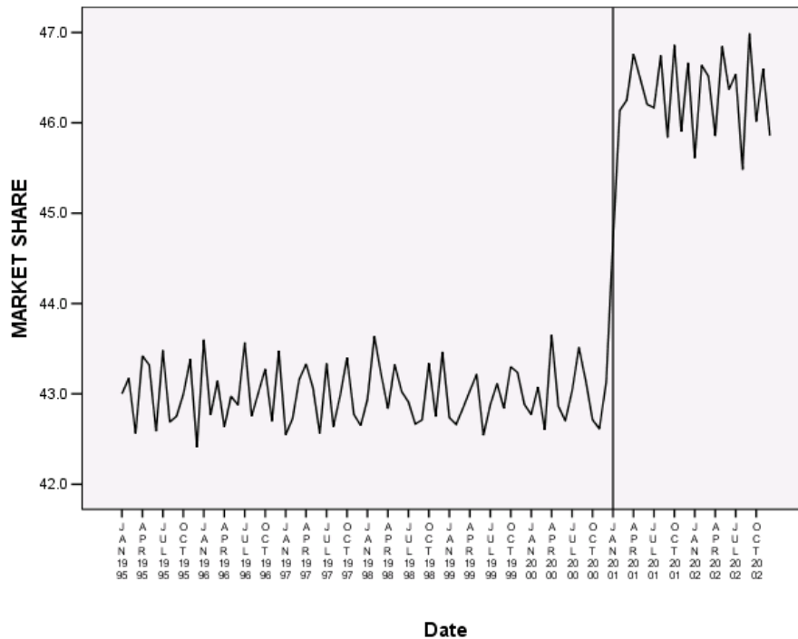
Figure 254-5 MARK=Y 2001 M 1
