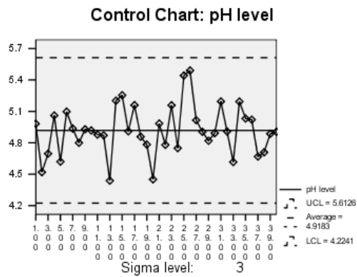
Figure 233-4 Individuals chart
