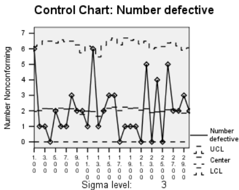
Figure 233-7 A np chart
