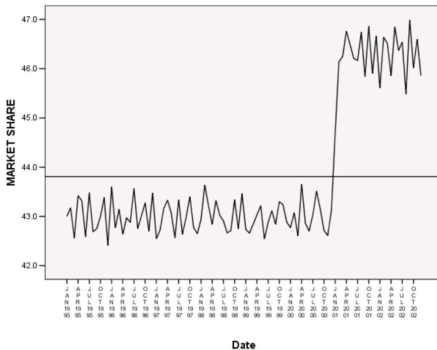
Figure 254-3 FORMAT=REFERENCE
