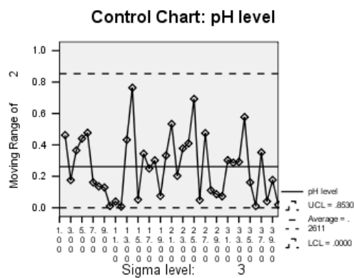
Figure 233-5 Moving range chart
