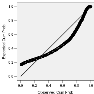
Figure 185-2 Normal p-p plot of household income
