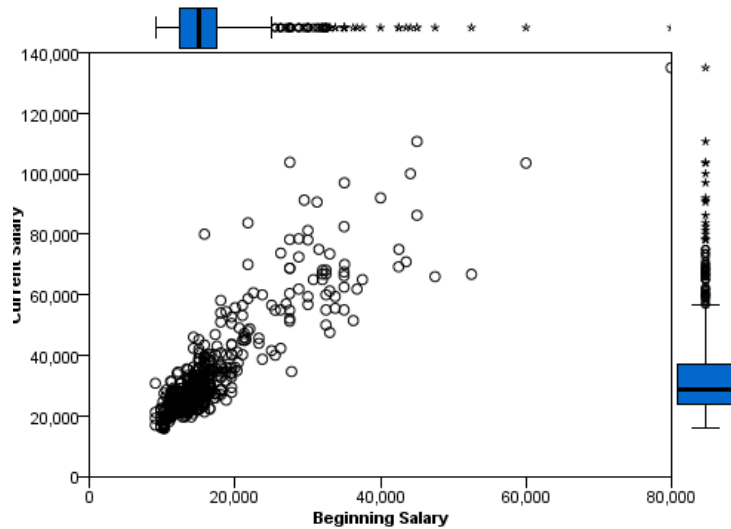
Figure 3-131 Scatterplot with border boxplots
