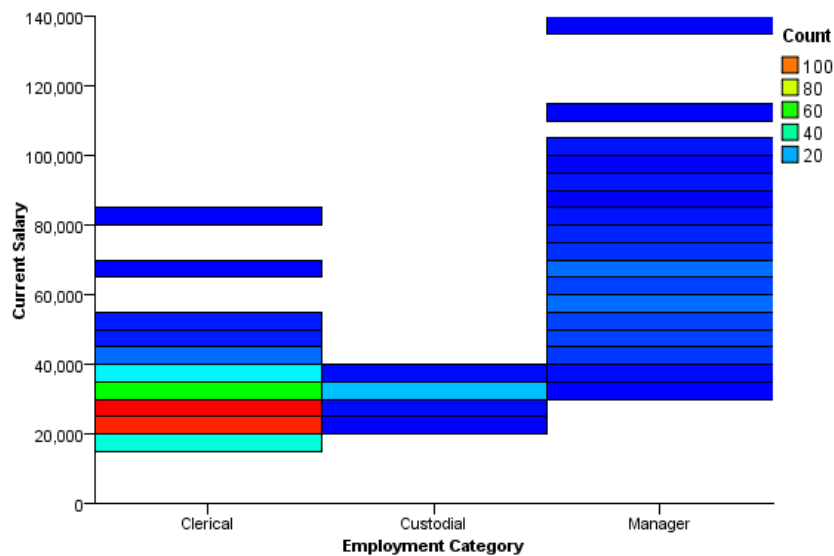
Figure 3-149 Binning over categorical values
