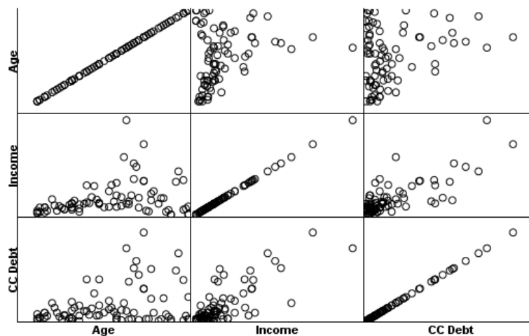
Figure 3-73 Scatterplot Matrix
