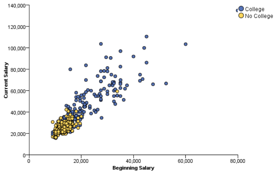
Figure 3-155
