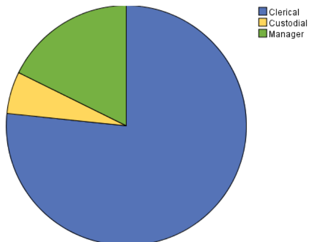
Figure 3-111 Pie chart
