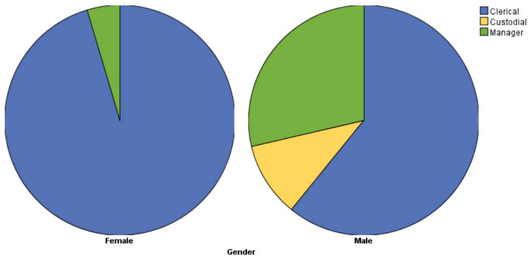
Figure 3-115
