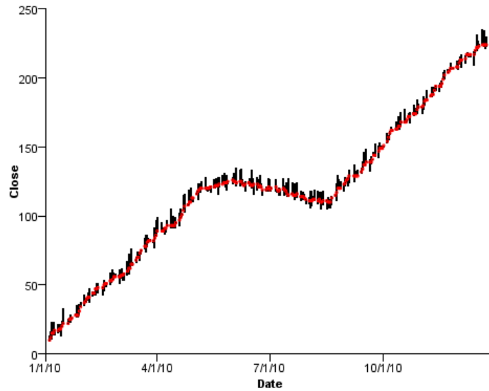
Figure 3-61 High-low-close chart
