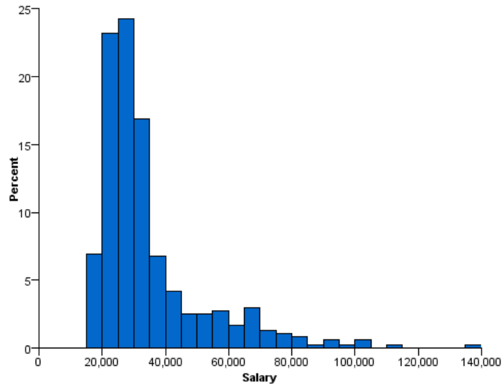
Figure 3-43 Percentage histogram
