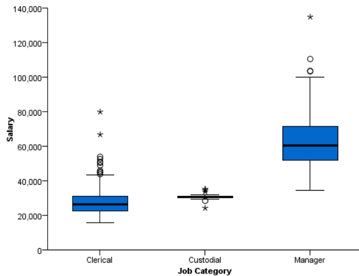
Figure 3-121 Boxplot
