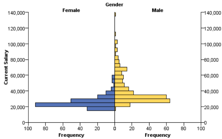
Figure 3-51 Population pyramid
