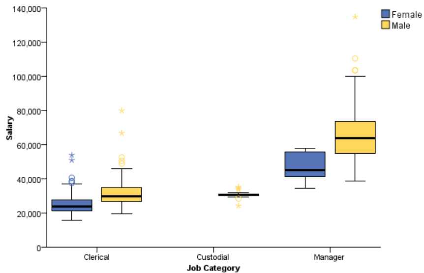
Figure 3-125 Clustered boxplot
