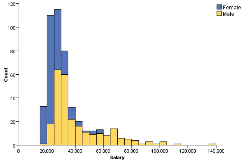
Figure 3-47 Stacked histogram
