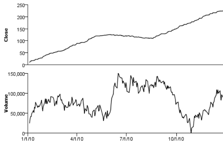
Figure 3-109
