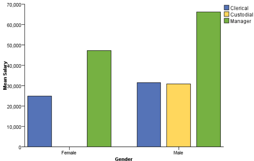
Figure 2-106
