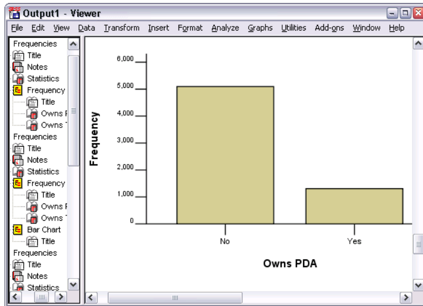
Figure 5-5 Bar chart
