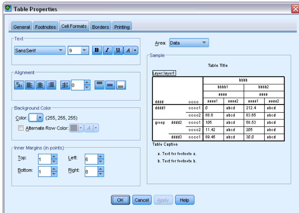
Figure 7-14 Table Properties dialog box
