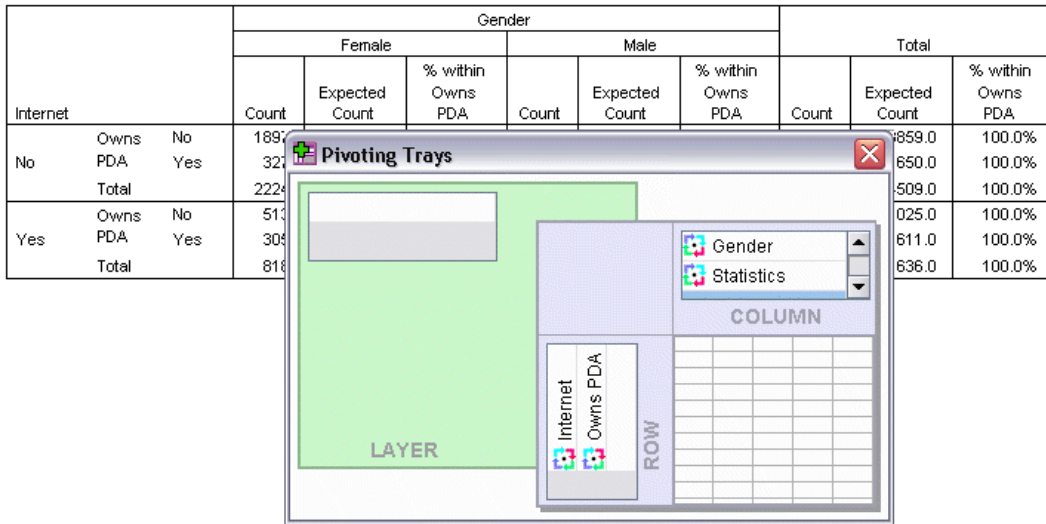
Figure 7-5 Moving rows to columns
