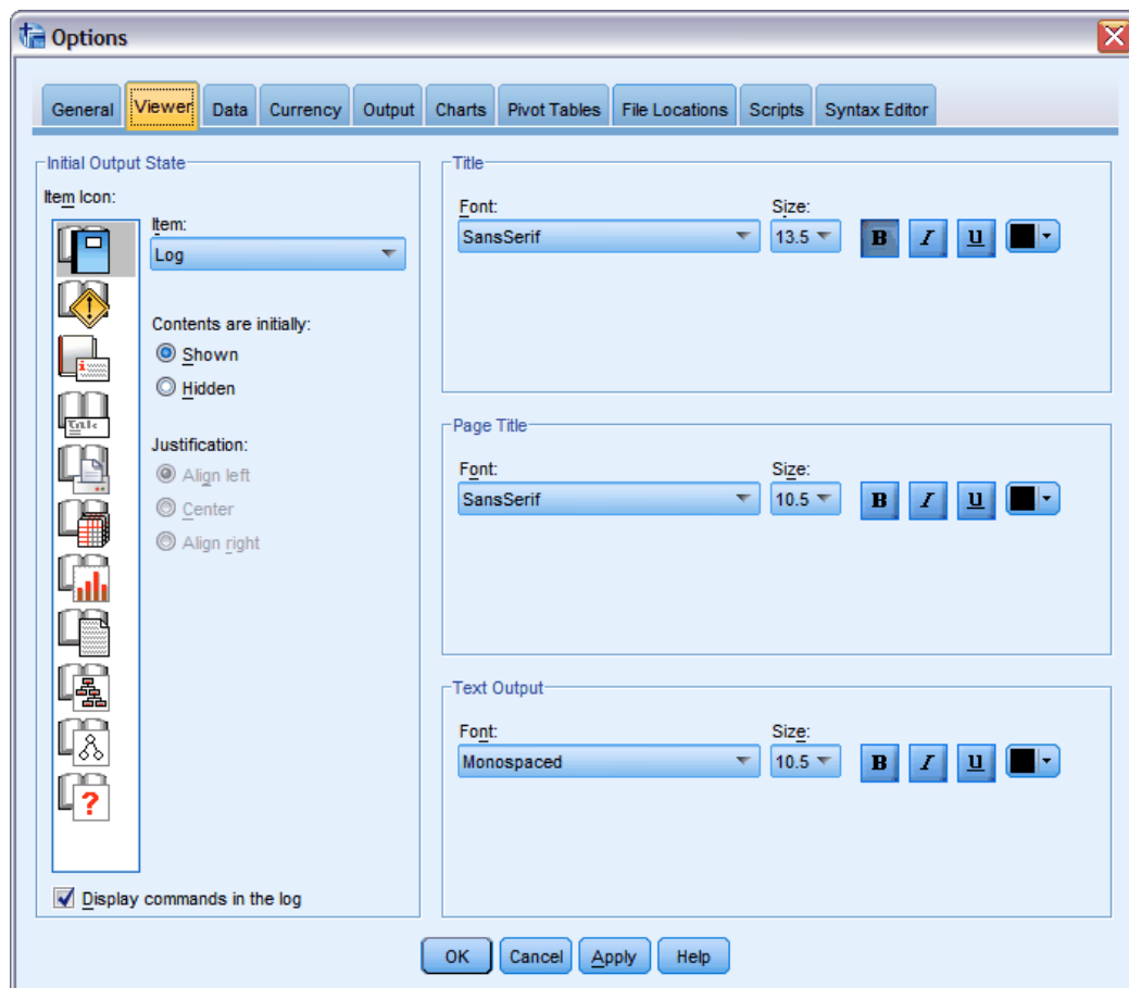
Figure 7-18 Viewer options
