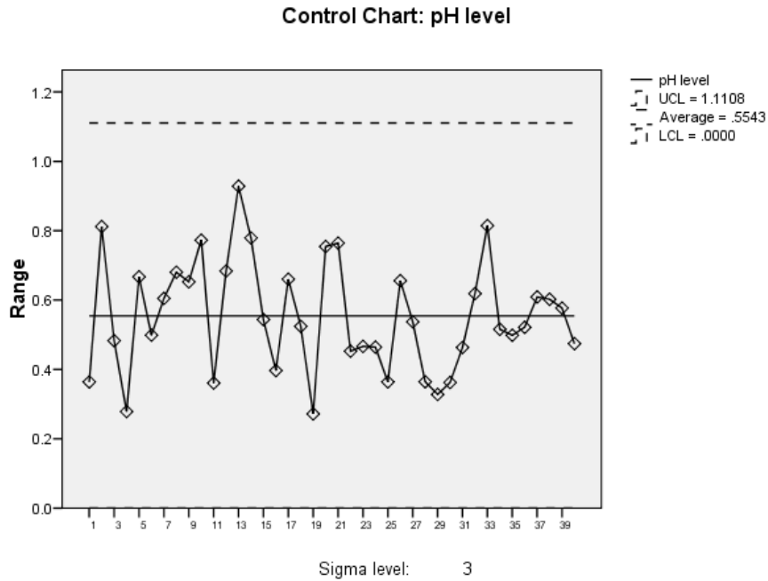
Figure 238-2 R chart
