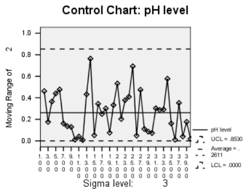
Figure 238-5 Moving range chart
