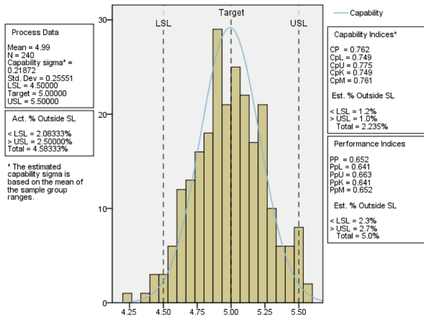
Figure 238-10 Process capability chart
