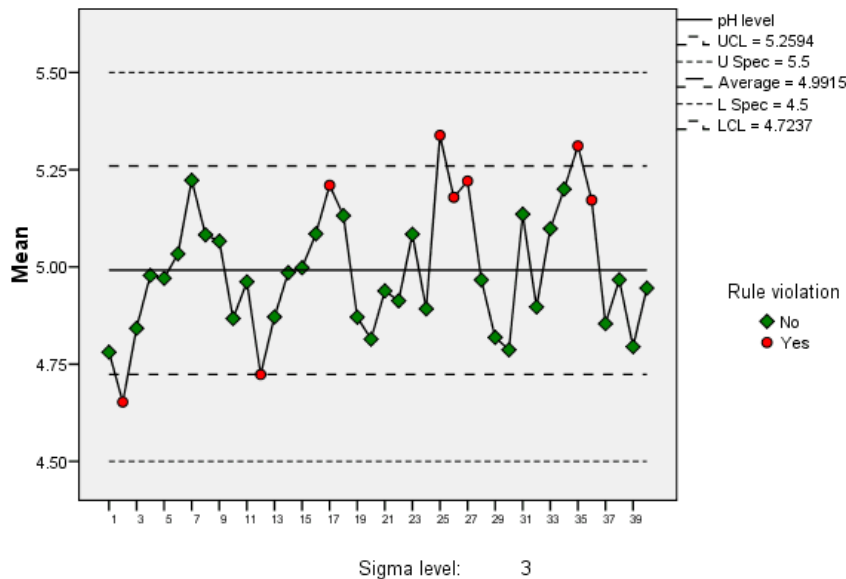
Figure 238-1 X-bar chart
