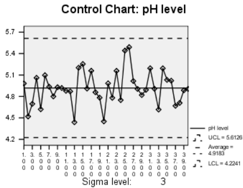
Figure 238-4 Individuals chart
