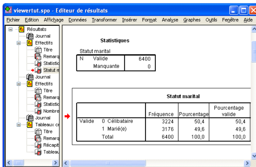
Figure 7-1 Viewer
