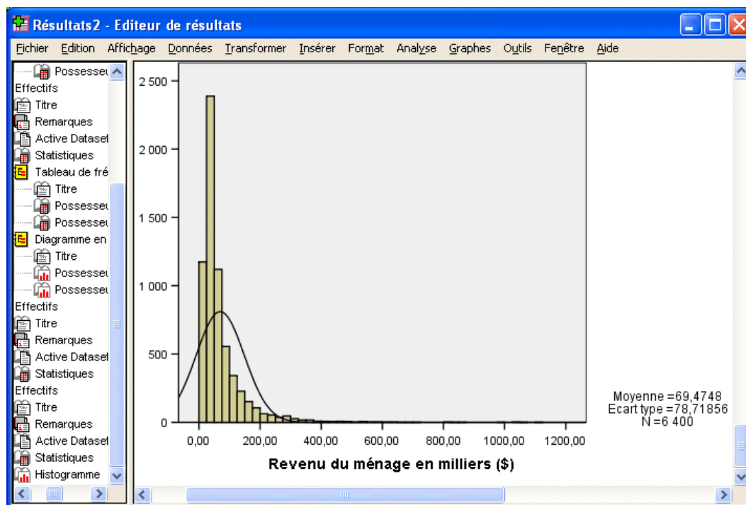
Figure 5-10 Histogramme
