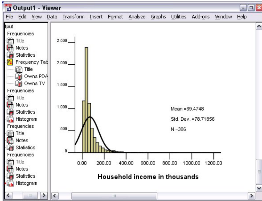
Figure 29. Histogramme
