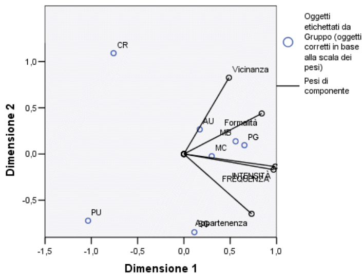
Figura 10-14 Biplot
